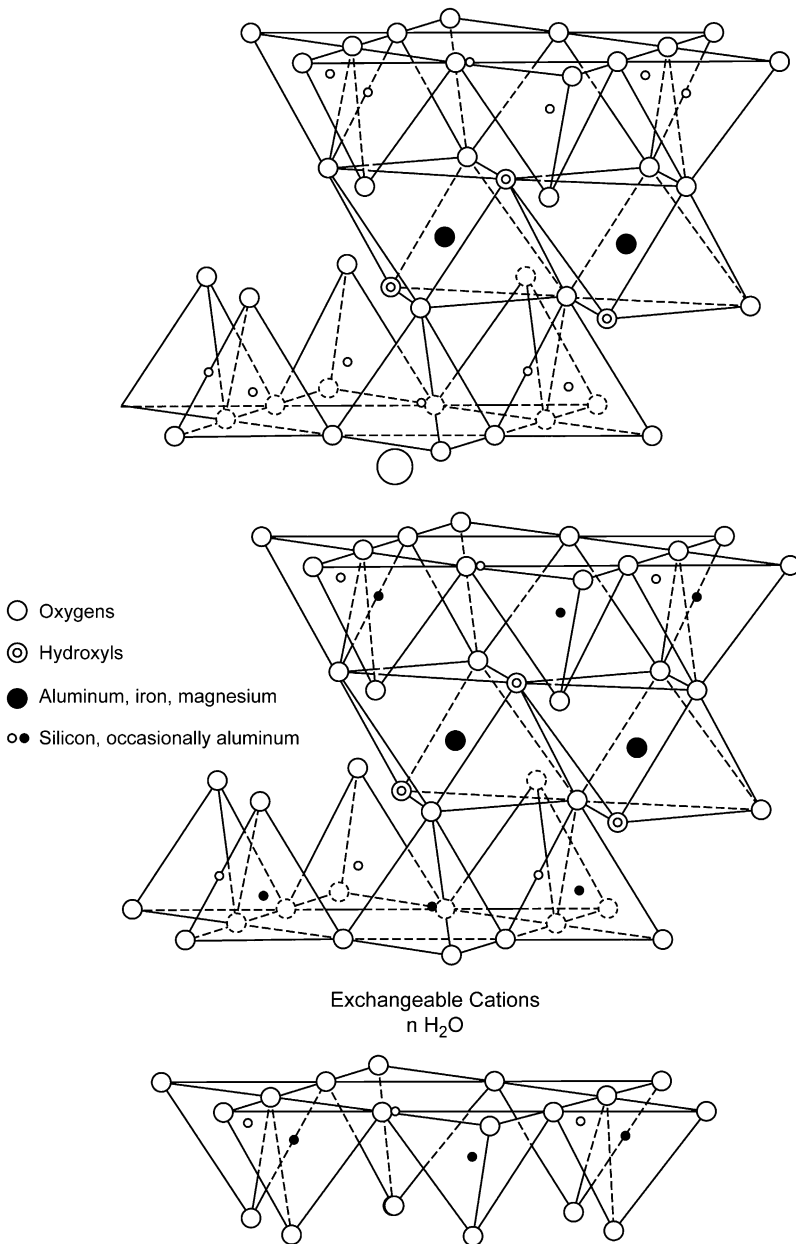
Fig. 18. Diagrammatic sketch of mixed-layer illite and smectite.
