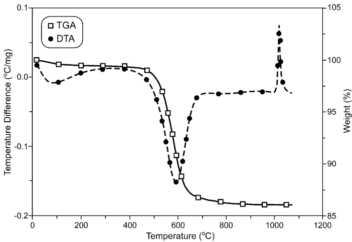
Fig. 60. Typical DTA–TGA curves of kaolinite showing the endothermic and exothermic reactions.
