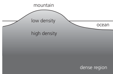
Pratt model
