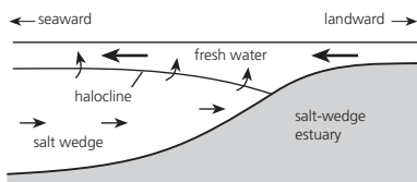
Salt wedge
