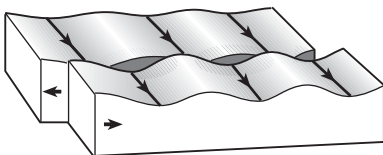
Shutter ridge
