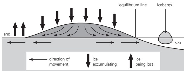
Ice sheet (cross section)
