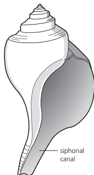
Siphonal canal
