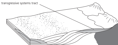
Transgressive systems tract
