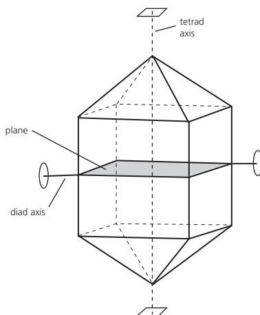
Crystal symmetry
