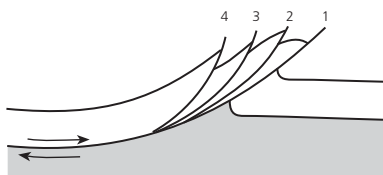
Break-back thrust
