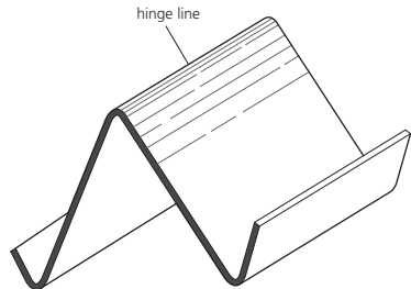
Hinge line
