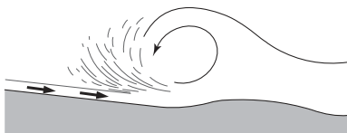
Plunging breaker
