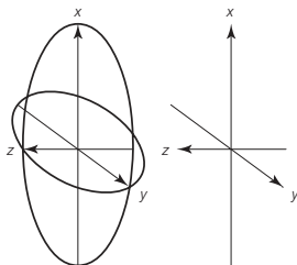
Strain ellipsoid
