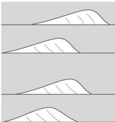
Lenticular bedding
