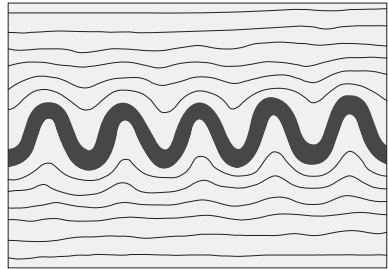
Buckle folding
