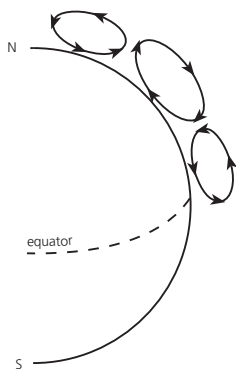
Three-cell model
