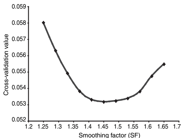
Figure 8.1 Ordovician–Silurian spline-curve cross-validation.
