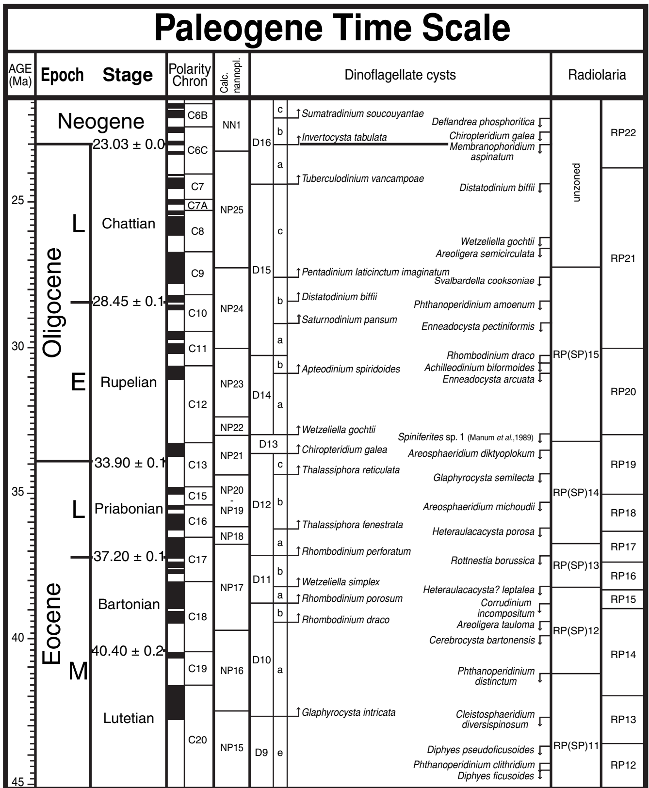
Figure 20.3 Paleogene dinoflagellate cyst zonation and datums and radiolarian zonation, with their estimated correlation to magnetostratigraphy and calcareous nannoplankton zones.
