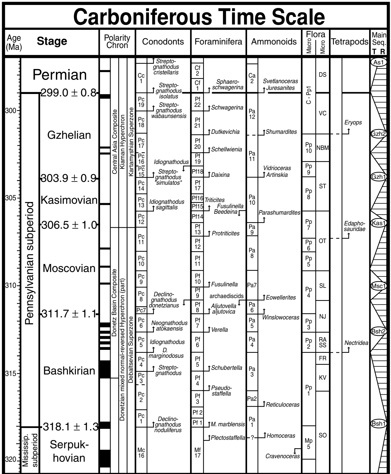
Figure 15.1 Subperiod and stage boundaries for the Carboniferous Period, with pelagic zonations of conodonts, foraminifera and ammonoids, and with terrestrial facies zonations of vertebrates, spores, and plants. The geomagnetic polarity scale with
