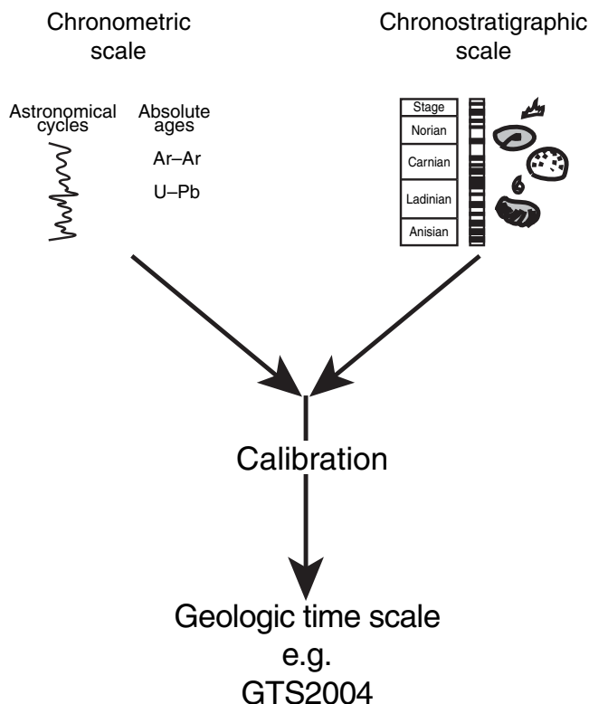
Figure 1.1 The construction of a geologic time scale is the merger of a chronometric scale (measured in years) and a chronostratigraphic scale (formalized definitions of geologic stages, biostratigraphic zonation units, magnetic polarity zones, and other subdivisions of the rock record).
