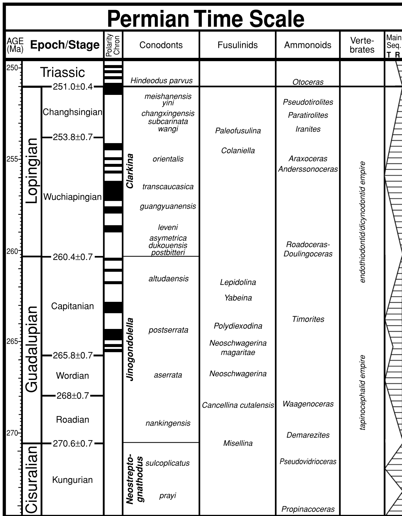
Figure 16.1 Permian time scale and magnetic polarity, conodont, fusulinid, ammonoid, vertebrate zonations, and general transgressive–regressive sequences. Magnetic polarity scale compiled from Irving (1963), Khramov, (1963), Peterson & Nairn
