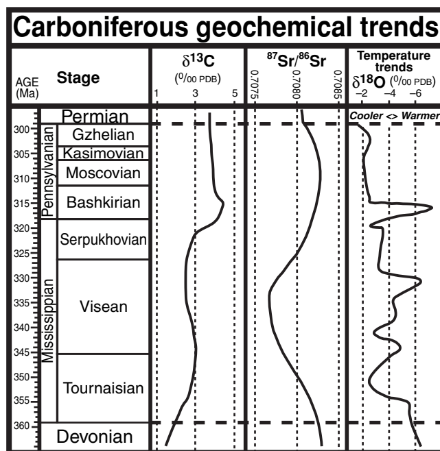
Figure 15.3 Geochemical trends during the Carboniferous Period. The schematic carbon isotope curve is a 5-Myr averaging of global data (Veizer et al. , 1999) from Hayes et al. (1999; downloaded from www.nosams.who.edu/jmh ). The ^{87}\text{Sr}/^{86}\text{Sr} LOWESS curve for the interval is based on the data of Denison et al. (1994) and other sources – see Chapter 7. The oxygen isotope curves (inverted scale) are derived from a 3-Myr interval averaging of global data compiled by Veizer et al. (1999; as downloaded from www.science.uottawa.ca/geology/isotope_data/ in January 2003). Large-scale global shifts to higher oxygen-18 values in carbonates generally are interpreted as cooler seawater or glacial episodes, but there are many other contributing factors (e.g. Veizer et al. , 1999, 2000; Wallmann, 2001).
