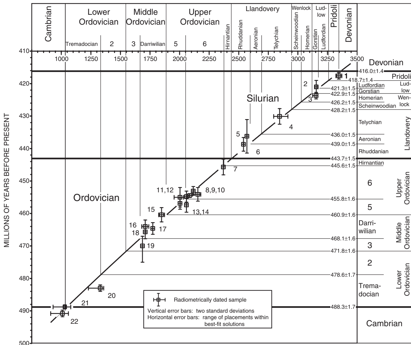
Figure 12.5 Graph showing the principle of constructing the Ordovician and Silurian time scale, using a plot of radiometric age dates for Late Cambrian through Silurian against the CONOP ordinal sequence of global graptolite events, which is compiled in Table 12.2. The numbers of the dates correspond to those listed in Table 12.1. Vertical error bars represent 2 standard deviations; horizontal error bars depict range of placement within best-fit solution. Although the best-fit line shown in this graph is a regression line with very slight curvature ( R^2 = 0.99 ), the final calculations that yielded the ages on Ordovician and Silurian stage
