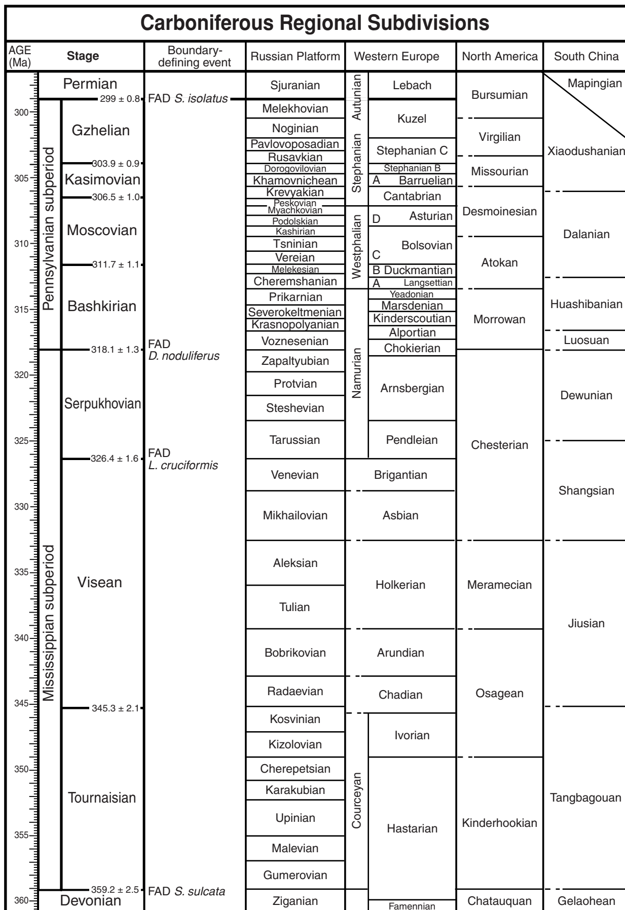
Figure 15.2 Correlation of regional Carboniferous stages and other stratigraphic subdivisions.
