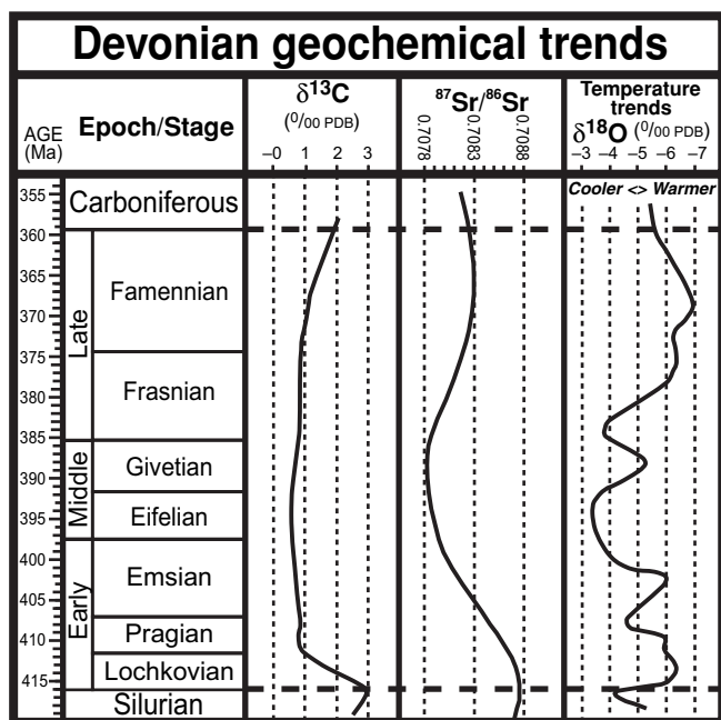
Figure 14.3 Geochemical trends in the Devonian Period. The schematic carbon isotope curve is a 5-myr averaging of global data (Veizer et al. , 1999) from Hayes et al. (1999; downloaded from www.nosams.who.edu/jmh ). The ^{87}\text{Sr}/^{86}\text{Sr} LOWESS curve for the interval is based on the data of Denison et al. (1997) and Carpenter et al. (1991) – see Chapter 7. The oxygen isotope curves (inverted scale) are derived from a 3-myr interval averaging of global data compiled by Veizer et al. (1999; as downloaded from www.science.uottawa.ca/geology/isotope_data/ in Jan 2003). Large-scale global shifts to higher oxygen-18 values in carbonates are generally interpreted as cooler seawater or glacial episodes, but there are many other contributing factors (e.g., Veizer et al. , 1999, 2000; Wallman, 2001).
