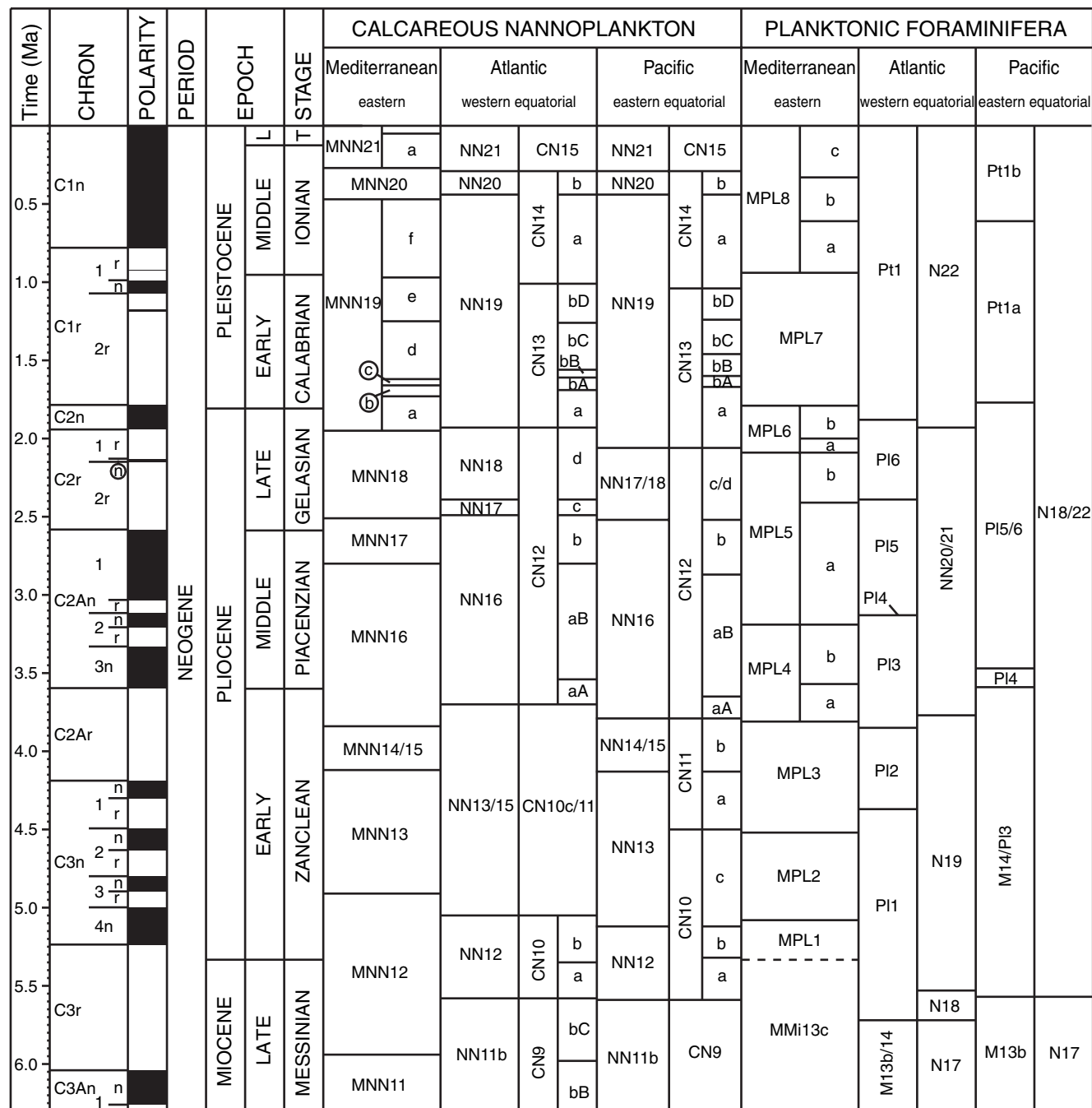
Figure 21.6 Correlation of planktonic foraminifer and calcareous nannoplankton zonal schemes for the Mediterranean, Atlantic, and Pacific. Astronomically tuned ages are based on Tables A2.1 through
