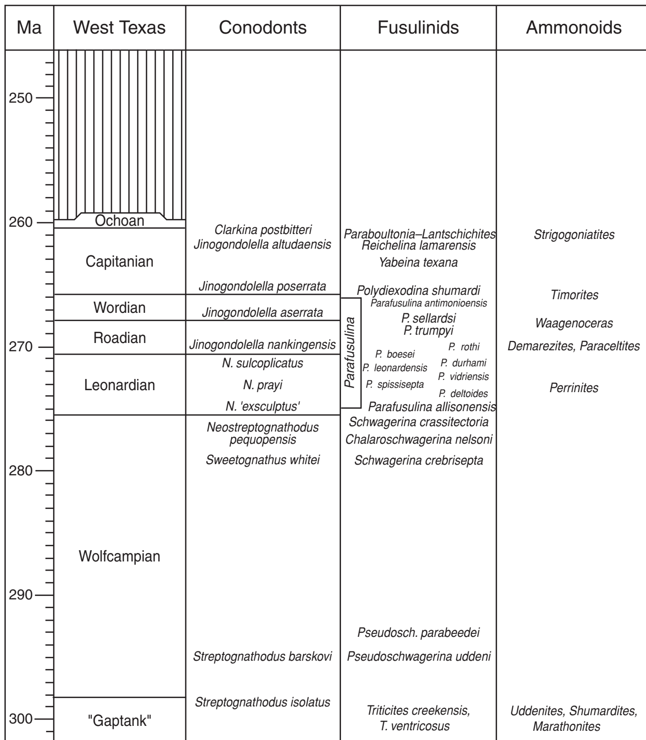
Figure 16.7 Regional correlation chart for West Texas with conodont, fusulinid, and ammonoid zonation.
