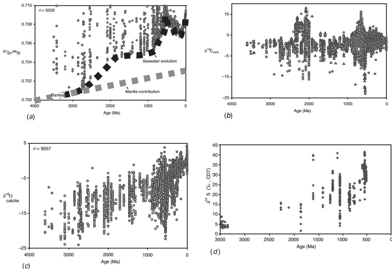
Figure 9.2 Strontium (a), carbon (b), oxygen (c), and sulfur (d) isotope geochemistry of marine carbonate and evaporite minerals through Earth history (modified after Shields and Veizer, 2002; Strauss, 2001a). Phanerozoic data are from Veizer et al. (1999). In Fig. 9.2(a–c), the filled symbols represent samples that are
