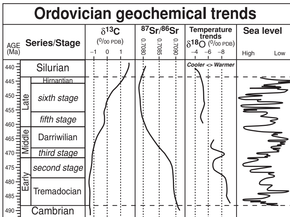
Figure 12.3 Geochemical and sea-level trends in the Ordovician Period. The schematic carbon isotope curve is a 5-myr averaging of global data (Veizer et al. , 1999) from Hayes et al. (1999; downloaded from www.nosams.who.edu/jmh ). The ^{87}\text{Sr}/^{86}\text{Sr} LOWESS curve for the interval is based on the data of Qing et al. (1998), Denison et al. (1998), and Ebner et al. (2001) – see Chapter 7. The oxygen isotope curves (inverted scale) are derived from a 3-myr interval
