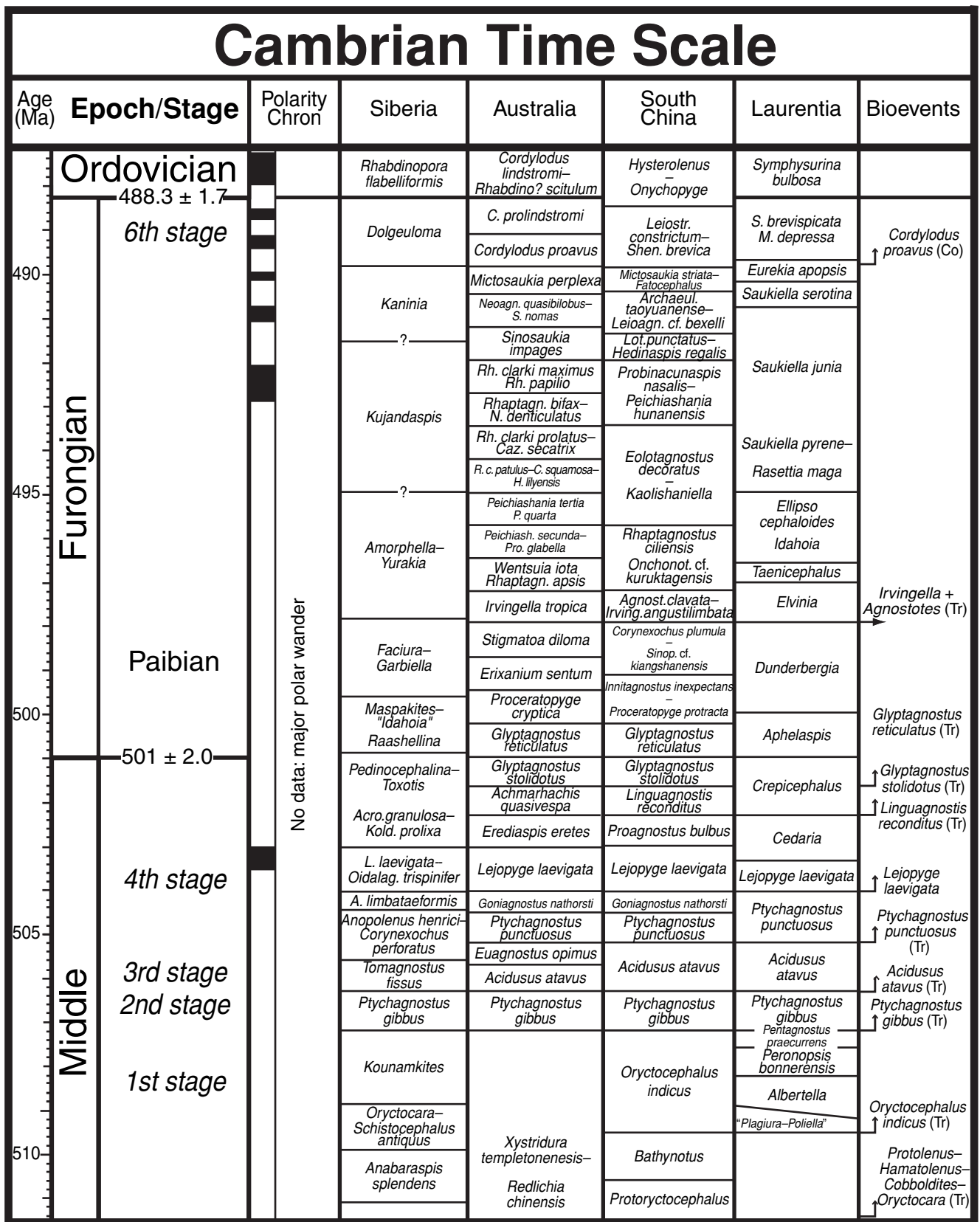
Figure 11.2 Principal biostratigraphic zonal schemes of the Cambrian. A color version of this figure can be found in the plate section.
