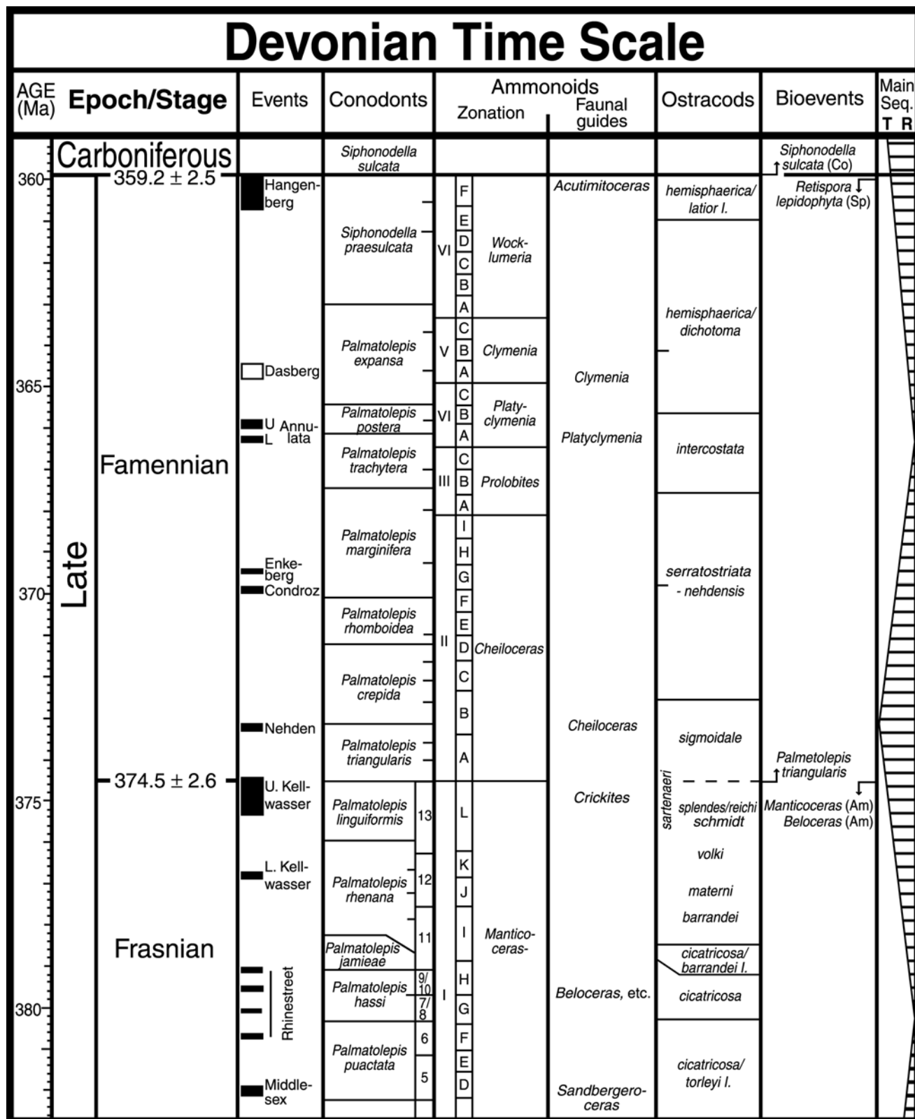
Figure 14.1 Epoch and stage boundaries and major marine biostratigraphic zonations for the Devonian Period with significant “event” levels (e.g. widespread anoxic facies or important outcrops) and principal eustatic trends. Biostratigraphic scales include conodonts, ammonoid zonation with selected guide taxa, graptolites,
