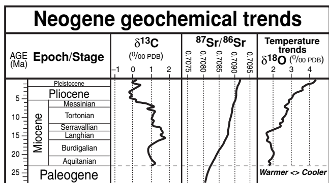
Figure 21.3 Generalized oxygen, carbon, and strontium isotope trends for the Neogene. See text for sources of oxygen and carbon curves. Strontium curve is a LOWESS fit to data from several sources (see text and Chapter 7).
