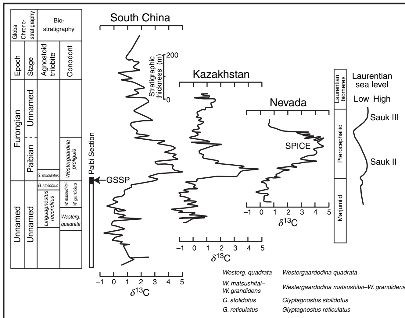
Figure 11.3 Correlation of basal-Paibian events with trends in \delta^{13}\text{C} and sea level.
