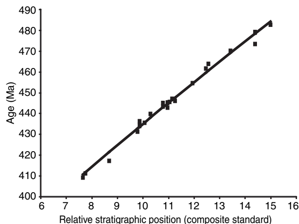
Figure 8.2 Ordovician–Silurian time scale: observed versus estimated values.
