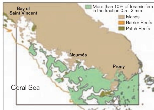
Figure 7 Contribution of foraminifera to the coarser ( > 0.5 \text{ mm} ) fraction of the sediment (after DEBENAY, 1985a).
