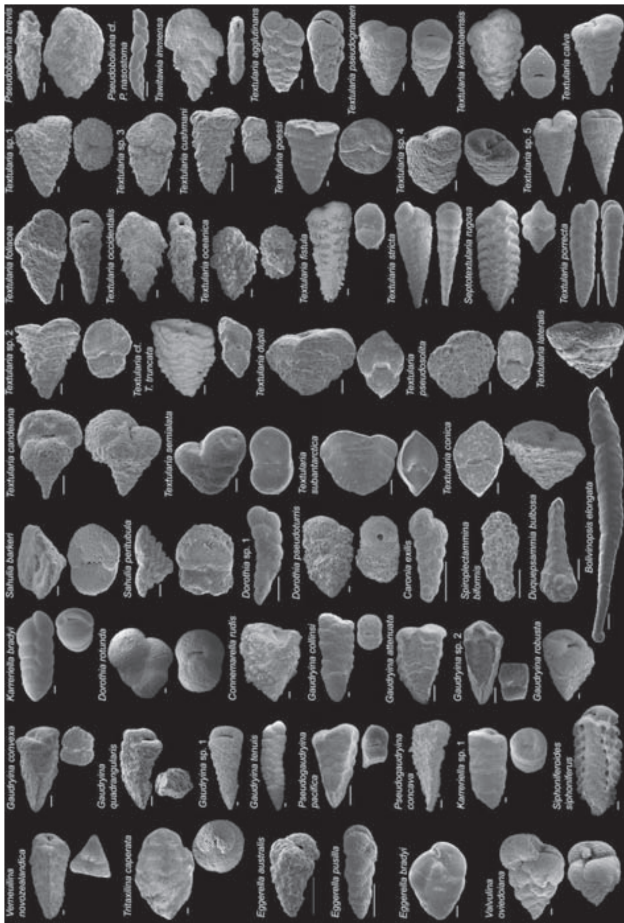
Plate 2 Agglutinated species. Scale bar = 0.1 mm.
