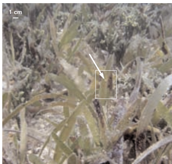
Figure 22 Living Marginopora vertebralis on sea grass (the arrow indicates one of the tens of individuals).
