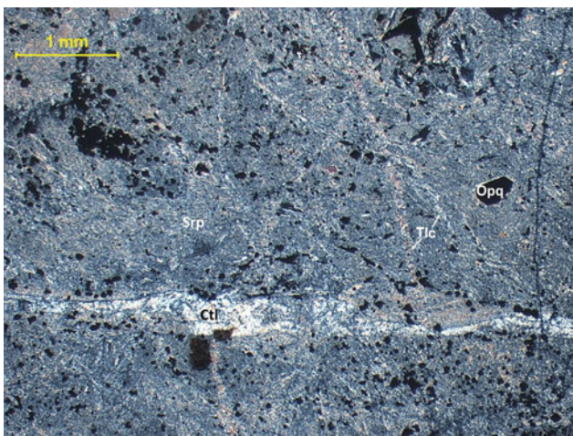
Plate Rd-1 Rodingite between crossed polars showing an opaque-talc-serpentine intergrowth traversed by veins of chrysotile and talc (70/79-2)
