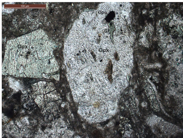
Plate Ptb-5 Magnified view of pleochroic orthopyroxene (neutral to green) and clinopyroxene (d, refer to Ptb-1) occurring as a girdle around rhyolite C21/79-4. The hypersthene contains inclusions of green and brown glass and opaque (C21/79-5)
