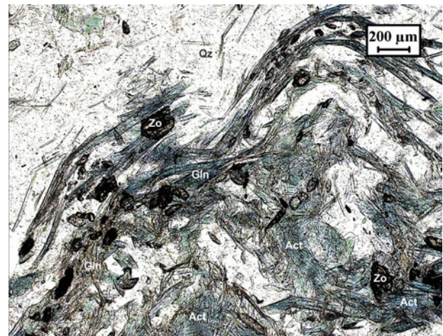
Plate Gln-33 Small warp in albite-phengite-actinolite-glaucophane schist with minor zoisite, magnetite and sphene in meta-arenite (ML-225-4)
