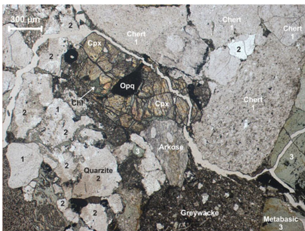
Plate Ptb-21 Tuff/epiclastic breccia between crossed polars showing sub-angular poorly sorted fragments of chert (1), quartzite (2), metabasite (3), arkose, pyroxenite and greywacke , and cross-cutting quartz vein. The rock is devoid of any matrix indicating little transport (84/80-1)
