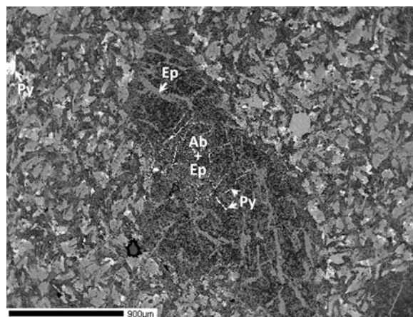
Plate V-20 Magnified backscattered electron image of a glomerocrystic aggregate of albite + epidote/zoisite pseudomorphs after plagioclase megacrysts with veins of epidote/zoisite and pyrite in metabasalt 371/79. The matrix is composed of an intergrowth of augite + epidote/albite + titanite (371/79)
