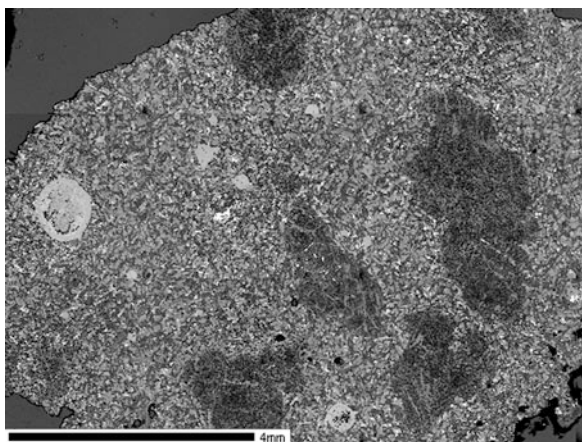
Plate V-19 Low magnification backscattered electron image of greenschist facies metabasalt with pseudomorphs after plagioclase megacrysts occurring in glomerocrystic aggregates and chlorite ocelli (371/79)
