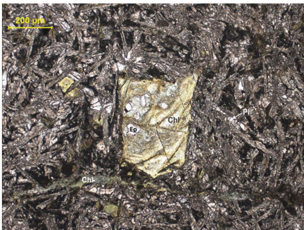
Plate V-1 Pseudomorph of chlorite + epidote after olivine phenocryst in porphyritic olivine basalt. The fine-grained groundmass shows an intersertal to intergranular texture (230/79-2)
