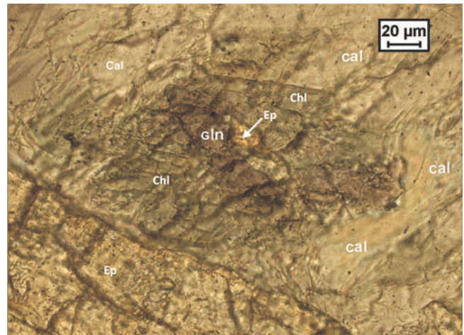
Plate Gln-7 Glaucophane-epidote intergrowth flanked by chlorite and surrounded by calcite and epidote porphyroblast in Ep-Chl-Ph-Gln-Omp schist (212/80-9)
