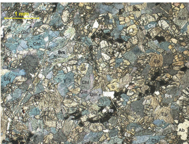
Plate Ec-1 Eclogite with granoblastic texture and an assemblage containing barroisite, glaucophane, chlorite, epidote, rutile, quartz and secondary albite (77/80-1)
