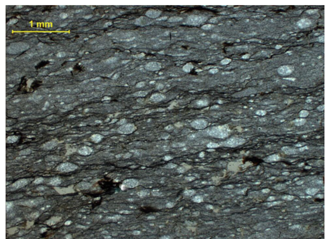
Plate OS_Ch-9 Tuffaceous chert showing radiolaria and fine biotite flakes along foliation. Crude crenulation is developed (Z55-1)
