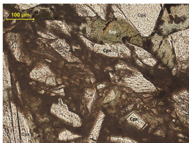
Plate SP-16 Brecciated non-pleochroic clinopyroxene and serpentine at the terminal part of micro-shear of spinel lherzolite in SP-15 showing protoclastic texture (96/80b-3)
