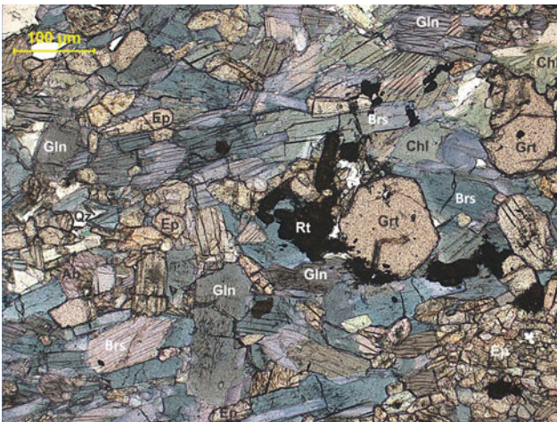
Plate Gln-23 Epidote-garnet-glaucophane-barroisite schist showing a granoblastic texture with minor garnet, phengite, rutile and late albite (139/79-1)
