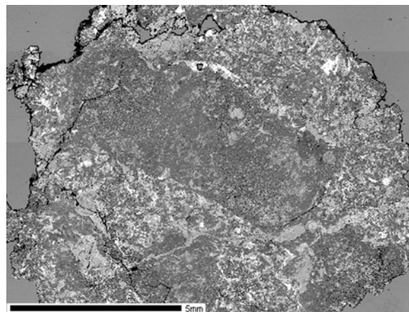
Plate V-29 Low magnification backscattered electron image of greenschist facies metabasalt with altered plagioclase megacrysts and chlorite-epidote veins (90/80)
