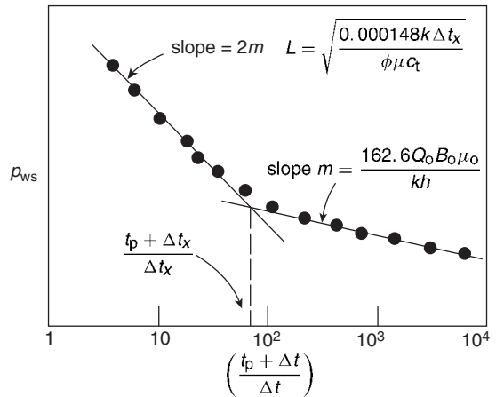
Figure 1.95 Theoretical Horner plot for a faulted system.
