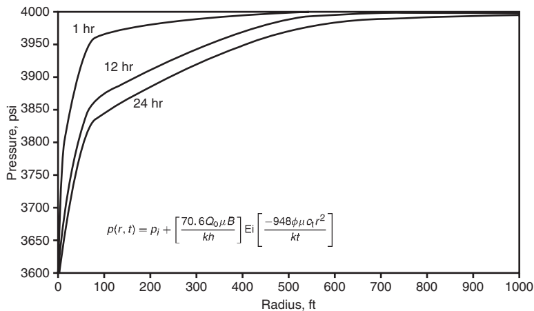
Figure 1.20 Pressure profiles as a function of time.
