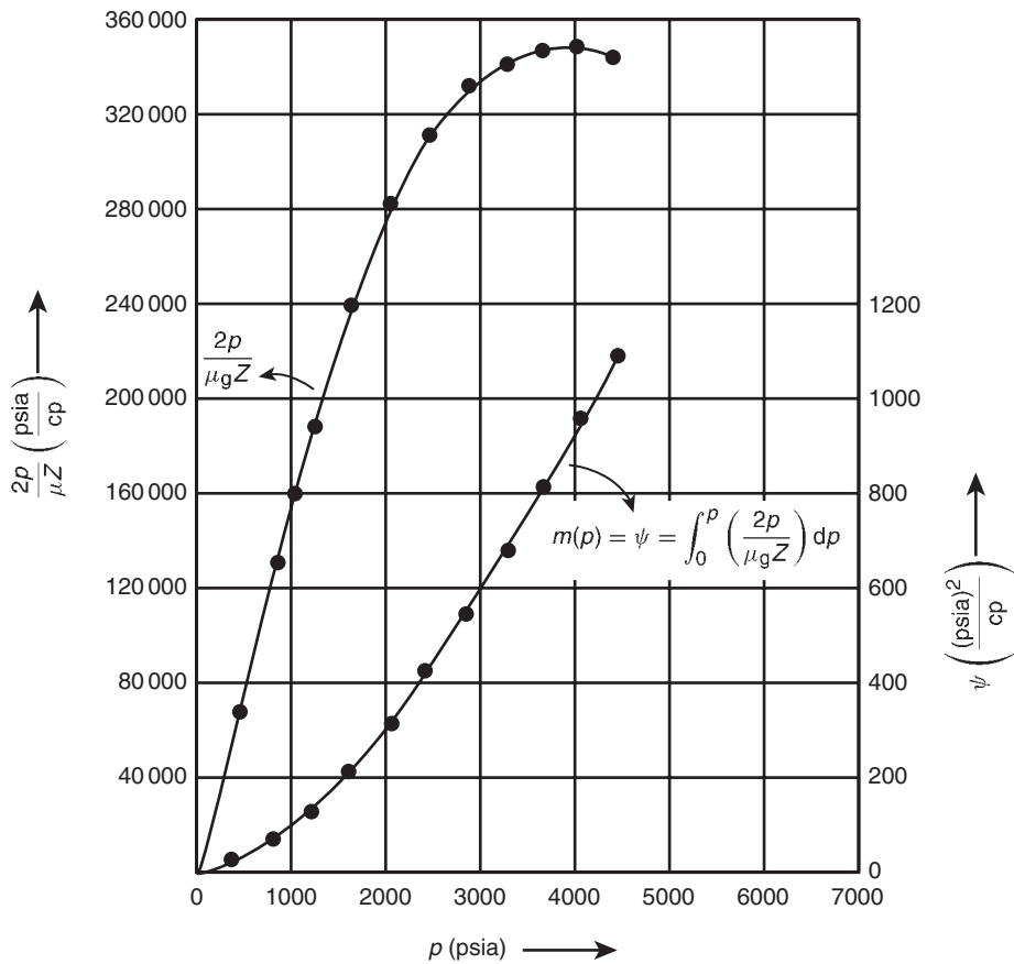
Figure 1.16 Real-gas pseudopressure data for Example 1.7 (After Donohue and Erekın, 1982).
