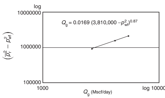
Figure 3.9 Back-pressure curve.
