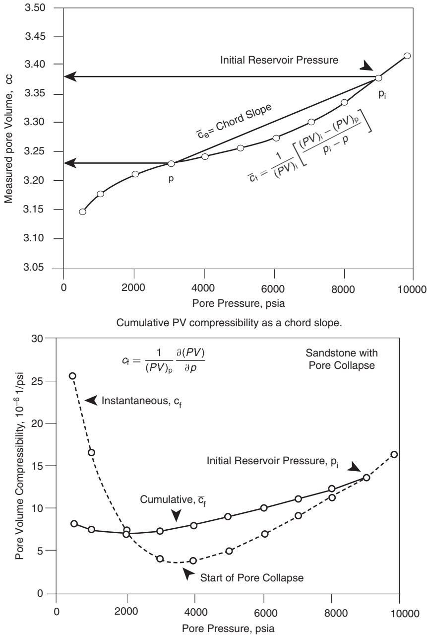
Figure 3.27 Cumulative and instantaneous c_f .
