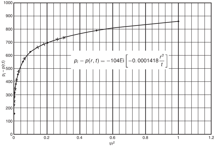
Figure 3.54 Pressure profile at 10 feet and 100 feet as a function of t/r^2 .
