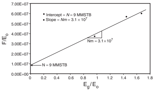
Figure 4.24 Calculation of m and N for Example 4.8.
