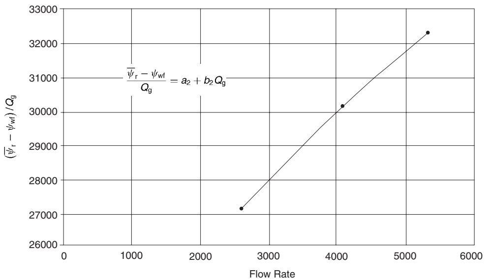
Figure 3.12 Pseudopressure method.
