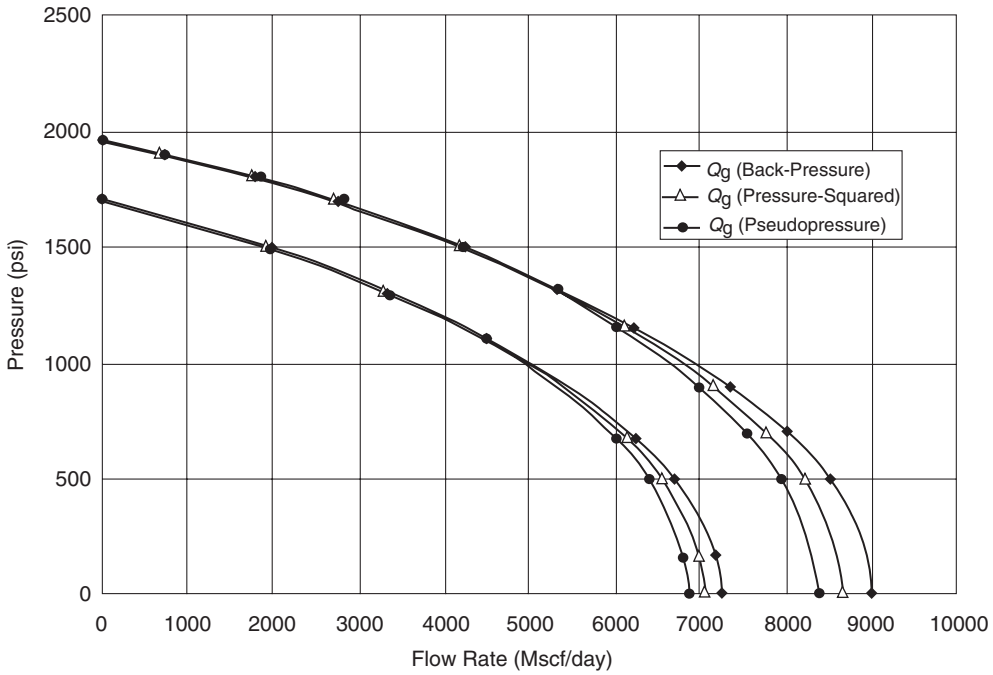
Figure 3.14 IPR comparison.
