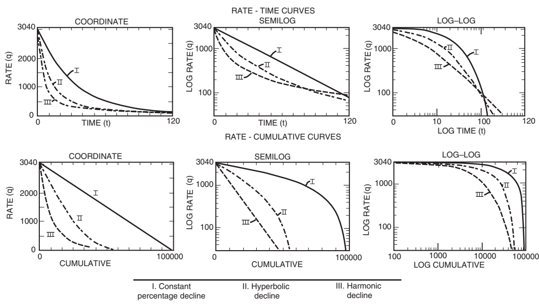
Figure 3.43 Classification of production decline curves. (After Arps, J.J. "Estimation of Primary Oil Reserves," Courtesy of Trans. AIME, vol. 207, 1956).
