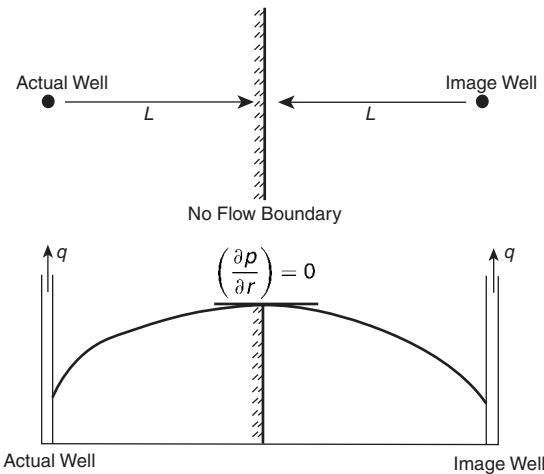
Figure 1.94 Method of images in solving boundary problems.
