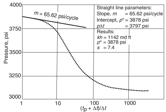
Figure 1.51 The Horner plot: data from Table 1.6 (Copyright ©1983 World Oil, Bourdet et al., May 1983).
