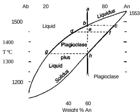
Figure 6-8 Isobaric T - X phase diagram for the albite-anorthite system at 0.1 MPa (atmospheric) pressure. After Bowen (1913). Reprinted by permission of the American Journal of Science.
