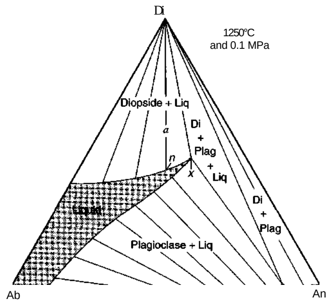
Figure 7-9 Isothermal section at 1250°C (and 0.1 MPa) in the system Di-An-Ab. From Morse (1994). Copyright © with permission from Krieger Publishers.
