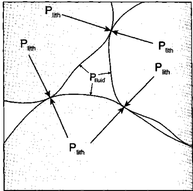
Figure 21-4 A situation in which lithostatic pressure exerted by the mineral grains is greater than the intergranular fluid pressure (/fluid)- At a depth around 10 km (or T around 300^{\circ}C ) minerals begin to yield or dissolve at the contact points and shift toward or precipitate in the fluid-filled areas, allowing the rock to compress. The decreased volume of the pore spaces will raise f_{fluid} until it equals P_{lith} .
