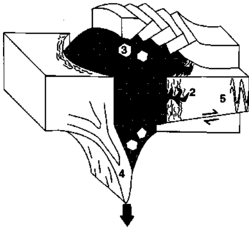
Figure 4-34 Diagrammatic illustration of proposed pluton emplacement mechanisms. (1) doming of roof; (2) wall rock assimilation, partial melting, zone melting; (3) stoping; (4) ductile wall rock deformation and wall rock return flow; (5) lateral wall rock displacement by faulting or folding; (6-) (and 1)- emplacement into extensional environment. After Pater-son et al. (1991). Copyright © the Mineralogical Society of America.
