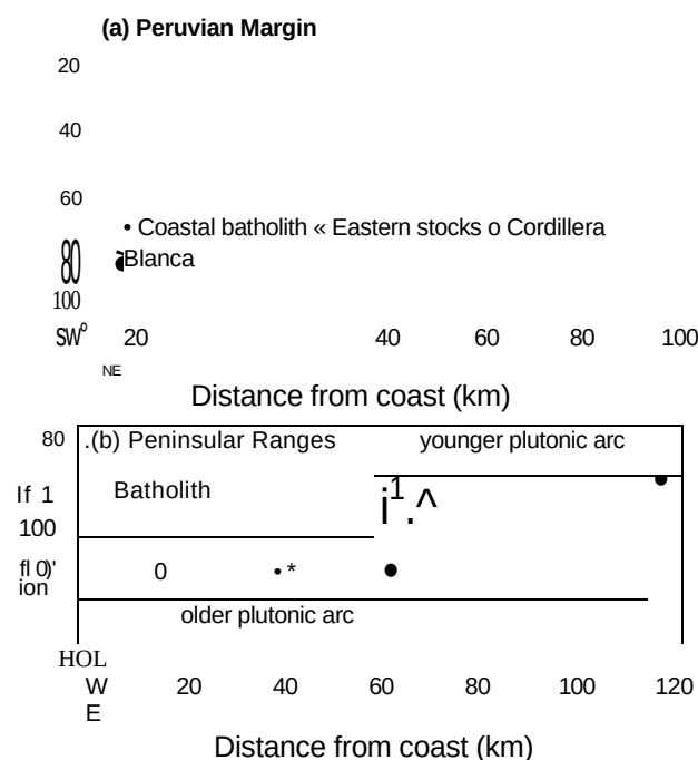
Figure 17-21 Isotopic age vs. distance across (a) the Western Cordillera of Peru (Cobbing and Pitcher, 1983) and (b) the Peninsular Ranges batholith of S. California/Baja Mexico (Walawender et al. 1990).
