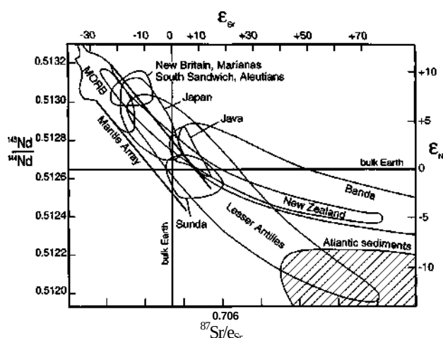
Figure 16-12 Nd-Sr isotopic variation in some island arc volcanics. MORB and mantle array from Figures 13-11 and 10-15. After Wilson (1989), Arculus and Powell (1986), Gill (1981), and McCulloch et al. (1994). Atlantic sediment data from White et al. (1985).
