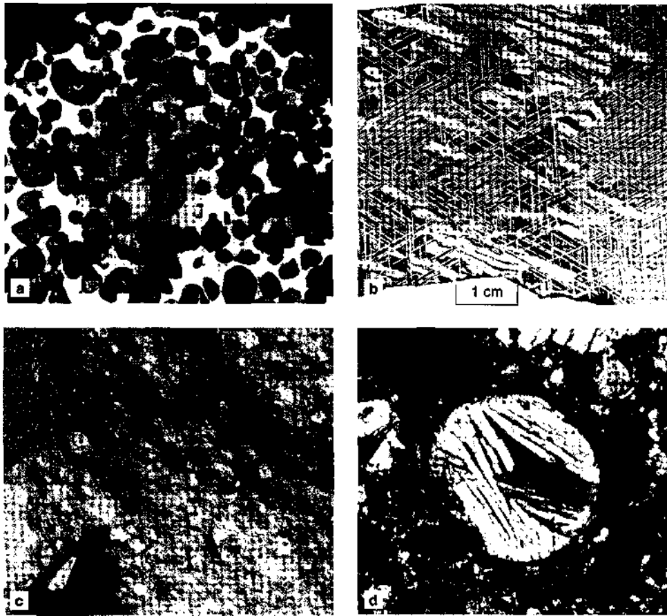
Figure 1-7 Meteorite textures, (a) Polished section of the stony-iron Springwater (Saskatchewan, Canada) meteorite (light is iron, dark is \sim 5\text{mm} olivines). © Courtesy Carleton Moore, Arizona State University, (b) Widmanstätten texture in the Edmonton (Kentucky) iron meteorite. © Courtesy John Wood and the Smithsonian Astrophysical Observatory, (c) Chondrules in the Allende chondrite meteorite (Mexico). Ball pen tip for scale, (d) Photomicrograph of a 0.5 mm diameter chondrule from the Dhajala (India) chondrite meteorite. The chondrule is composed of skeletal plates of olivine in a finer matrix including crystal fragments and glass. Other chondrules may be dominated by orthopyroxene, or mixtures of several minerals, including sulfides. Chondrules may be very fine grained or even totally glassy in meteorites that have suffered little or no reheating. Chondrite photographs courtesy of the Geological Museum, University of Copenhagen ©.
