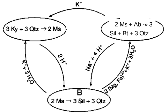
Figure 26-22 An alternative mechanism by which the reaction \text{Ky} \rightarrow \text{Sil} reaction can be accomplished while producing sillimanite needles associated with biotite whereas plagioclase occupies embayments in the biotite. The exchange of ions shown between the two local zones is required if the reactions are to occur. After Carmichael (1969). Copyright © with permission from Springer-Verlag.
