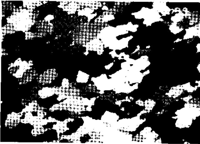
Figure 23-29 Deformed quartzite in which elongated quartz crystals following shear, recovery, and recrystallization. Note the broad and rounded suturing due to coalescence. Field width \sim 1 cm. From Spry (1969).
