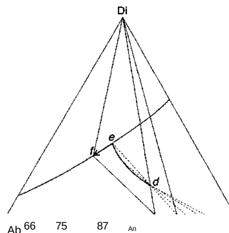
Figure 7-7 Liquid evolution path of bulk composition d ( \text{Di}_{30}\text{An}_{55}\text{Ab}_{15} ) in the diopside-anorthite-albite system at 0.1 MPa. The curvature of path d - e is exaggerated.
