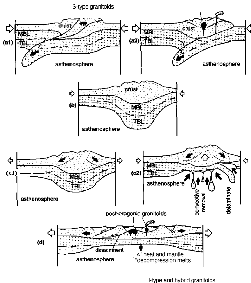
Figure 18-8 Schematic models for the uplift and extensional collapse of orogenically thickened continental crust. Subduction leads to thickened crust by either continental collision ( a1 ) or compression of the continental arc ( a2 ), each with its characteristic orogenic magmatism. Both mechanisms lead to a thickened crust, and probably thickened mechanical and thermal boundary layers ("MBL" and "TBL") as in ( b ). Following the stable situation in ( b ), either compression ceases ( c1 ) or the thick dense thermal boundary layer is removed by delamination or convective erosion ( c2 ). The result is extension and collapse of the crust, thinning of the lithosphere, and rise of hot asthenosphere ( d ). The increased heat flux in ( d ), plus the decompression melting of the rising asthenosphere, results in bimodal post-orogenic magmatism with both mafic mantle and silicic crustal melts.
