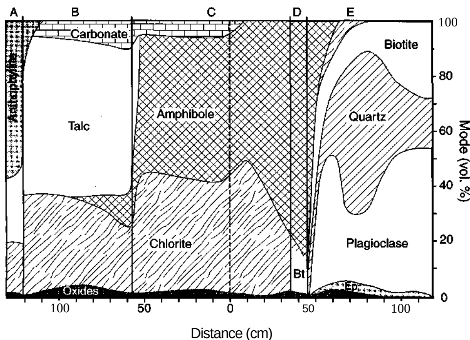
Figure 30-16 Variation in mineral proportions across the zones between the ultramafic and quartzzo-feldspathic gneiss contact at Grafton, Vermont, after Sanford (1982). Zone letters at the top correspond to the zones listed in the text. Zone letters at the top are: A = Tic + Ath, B = Tic, C = Act + Chi, D = transitional, E = quartzzo-feldspathic country rock. The vertical dashed line represents the estimated initial contact. After Sanford (1982). Reprinted by permission of the American Journal of Science.
