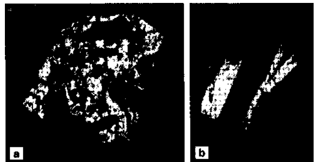
Figure 3-4 (a) Skeletal olivine phenocryst with rapid growth at edges enveloping melt at ends. Taupo, N.Z. (b) "Swallow-tail" plagioclase in trachyte, Remarkable Dike, N.Z. Length of both fields ca. 0.2 mm. From Shelley (1993). Copyright © by permission Kluwer Academic Publishers.
