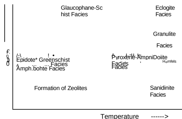
Figure 25-1 The metamorphic facies proposed by Eskola and their relative temperature-pressure relationships. After Eskola (1939).
