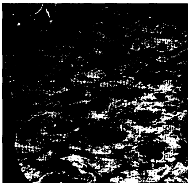
Figure 23-18 Augen gneiss with eye-shaped porphyroclasts (augen) of K-feldspar in a sheared granitic
