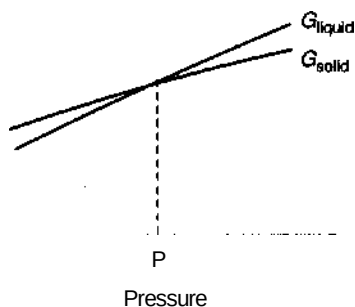
Figure 5-4 Relationship between Gibbs free energy and pressure for the solid and liquid forms of a substance at constant temperature. P_{eq} is the equilibrium pressure.
