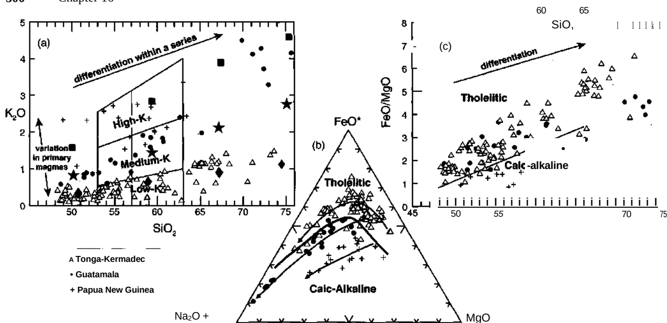
Figure 16-6 Variation in the Tonga-Kermadec, Guatemala, and Papua New Guinea volcanic suites, (a) K 2 O-SiO 2 diagram (after Gill, 1981, copyright © with permission from Springer-Verlag) distinguishing high-K, medium-K and low-K series. Large squares = high-K, stars = med.-K, diamonds = low-K series from Table 16-2. Smaller symbols are identified in the caption. Differentiation within a series (presumably dominated by fractional crystallization) is indicated by the arrow. Different primary magmas (to the left) are distinguished by vertical variations in K 2 O at low SiO 2 . (b) AFM diagram distinguishing tholeiitic and calc-alkaline series. Arrows represent differentiation trends within a series, (c) FeO*/MgO vs. SiO 2 diagram distinguishing tholeiitic and calc-alkaline series. Note that Tonga-Kermadec is both low-K and tholeiitic, PNG is high-K and calc-alkaline, whereas Central America is medium-K and calc-alkaline by the criteria of (b), but borderline by that of (c).
