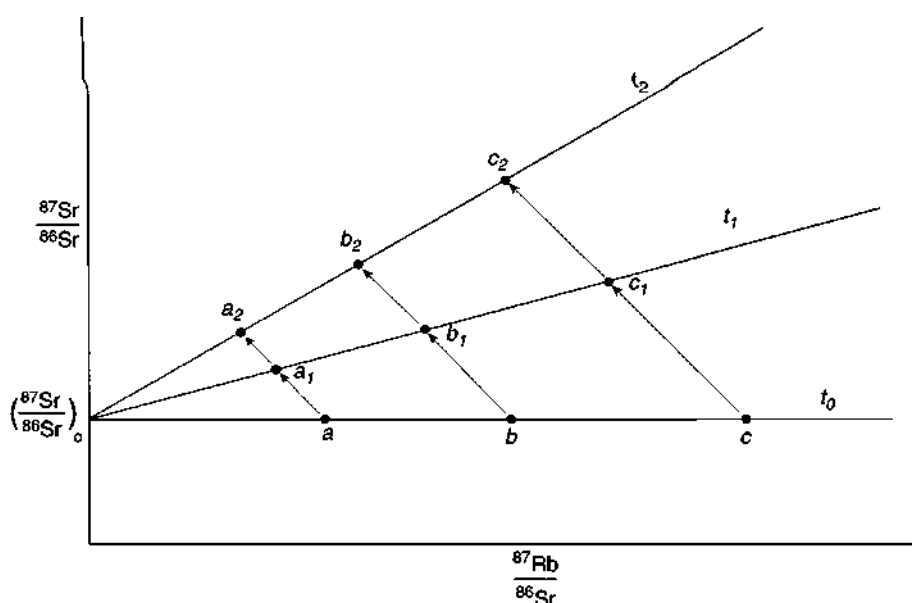
Figure 9-11 Schematic Rb-Sr isochron diagram showing the isotopic evolution over time of three rocks or minerals (a, b, and c) with different Rb/Sr ratios after their derivation from a homogeneous source at time t_0 .
