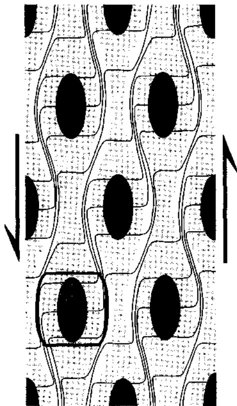
Figure 23-40 Non-uniform distribution of shear strain as proposed by Bell et al. (1986). Blank areas represent high shear strain and dark areas are low-strain. Lines represent initially horizontal inert markers ( S^\wedge ).
