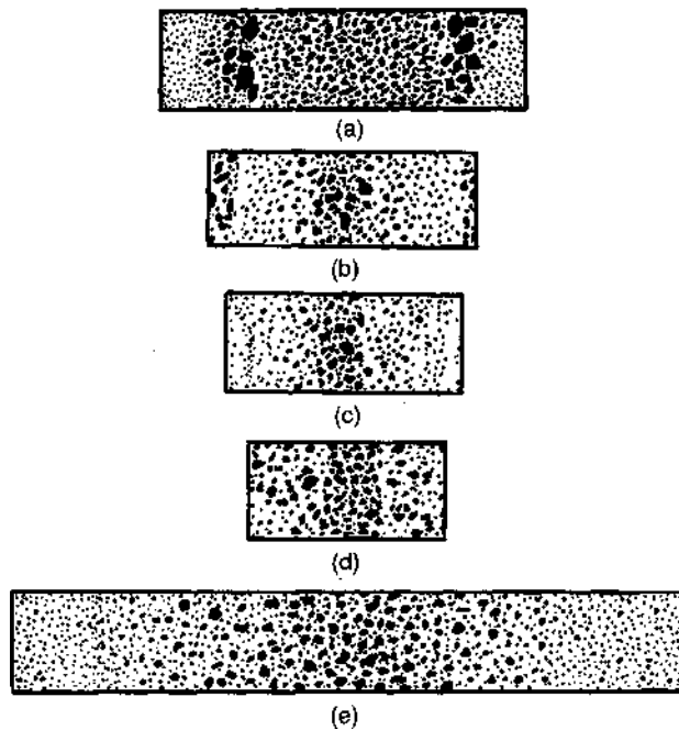
Figure 11-5 Increase in size and concentration of olivine phenocrysts toward the center of small dikes by flow differentiation, Isle of Skye, Scotland. After Drever and Johnston (1958). Reproduced by permission of the Royal Society of Edinburgh.
