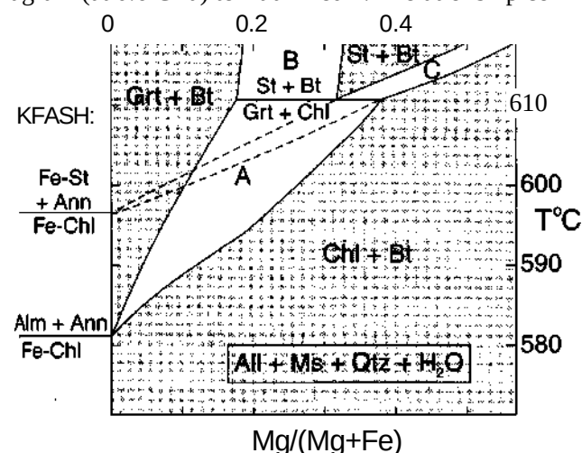
Figure 28-12 T-X_{\text{Mg}} "pseudosection" diagram in the system KFMASH of variable \text{Mg/Fe} for a "common pelite" with molar \text{Al:F:K} = 0.92:1:0.28 , calculated by Powell et al. (1998). I have modified the temperatures of the original isobaric diagram to conform with the specified medium P/T trajectory in Figure 28-2.
