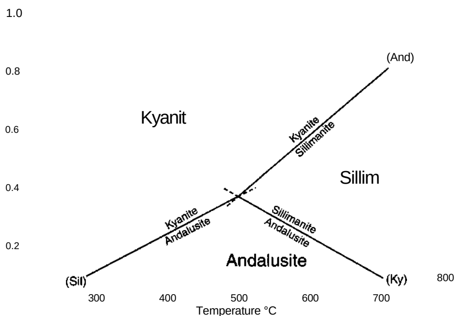
Figure 26-15 The \text{Al}_2\text{SiO}_5 T - P phase diagram from Figure 21-9 (without \text{H}_2\text{O} ).
