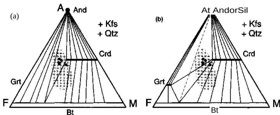
Figure 28-19 AFM diagrams (projected from Kfs) in the lowermost pyroxene hornfels facies , (a) The compositional range of cordierite is reduced as the Crd - And - Bt sub-triangle migrates toward more Mg-rich compositions. Andalusite may be introduced into Al-rich pelites (b) Garnet is introduced to many Al-rich pelites via Reaction (28-27).
