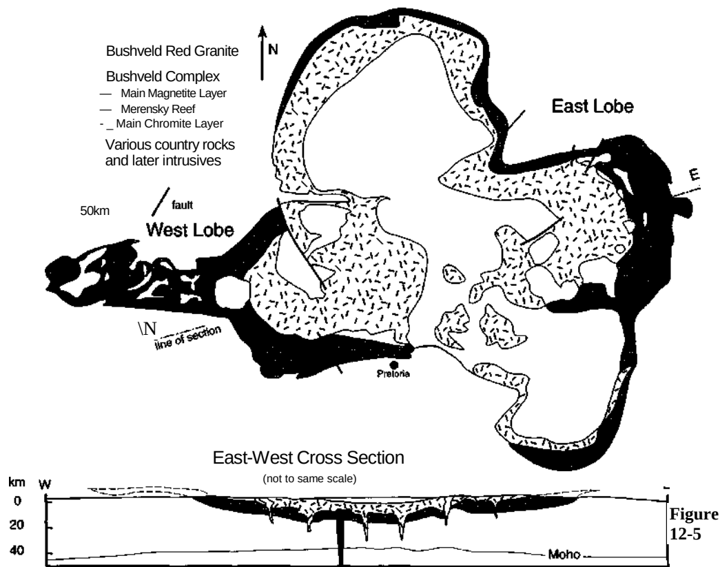
Simplified geologic map and cross section of the Bushveld complex. After Willemse (1964), Wager and Brown (1968), and Irvine et al. (1983).
