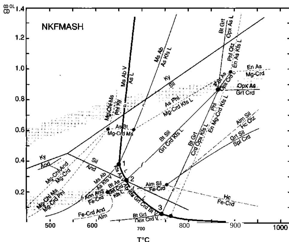
Figure 28-21 High-temperature petrogenetic grid showing the location of selected melting and dehydration equilibria in the \text{Na}_2\text{O}-\text{K}_2\text{O}-\text{FeO}-\text{MgO}-\text{Al}_2\text{O}_3-\text{SiO}_2-\text{H}_2\text{O} (NKFMASH) system, with sufficient sodium to stabilize albite. Also shown are some equilibria in the KFMASH (dotted) and KMASH (dashed) systems. Reactions are not balanced and commonly leave out Ms and Qtz, which are considered to be present in excess. The medium and low P/T meta-morphic field gradients from Figure 28-2 (broad shaded arrows) are included for comparative purposes. The \text{Al}_2\text{SiO}_5 triple point is shifted as shown to 550^\circ\text{C} and 0.45 GPa following the arguments of Pattison (1992), allowing for the coexistence of andalusite and liquid. V = \text{H}_2\text{O} -rich vapor, when present in fluid-saturated rocks. After Spear et al. (1999).
