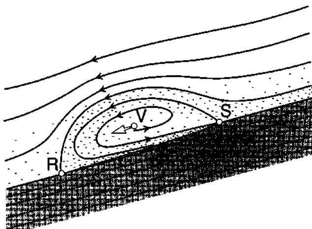
Figure 12-16 Cross section of a vortex cell in a density surge current along the boundary layer between floor cumulates (shaded) and magma. Streamlines and arrows portray the instantaneous flow relations relative to points V, R, and S. The floor is actually stationary, of course, and points V, R, and S move as shown with the arrow at V. Flow within the surge moves faster than the vortex (as in a tractor tread), so that the flow material separates from the floor at S and reattaches at R. Forward motion of the vortex results in deposition between it and the chamber floor. After Irvine et al. (1999). Copyright © The Geological Society of America, Inc.
