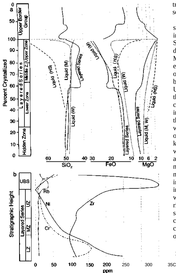
Figure 12-13 Variation in selected major (a) and trace elements (b) in the Skaergard Intrusion. Major elements are determined for the Layered Series and Upper Border Series, as well as calculated for hypothetical liquids based on the models of McBirney, 1975 (M), Wager, 1960 (W), and Hunter and Sparks, 1987 (HS). After McBirney (1993). Jones and Bartlett Publishers, Sudbury, MA. Reprinted with permission.
