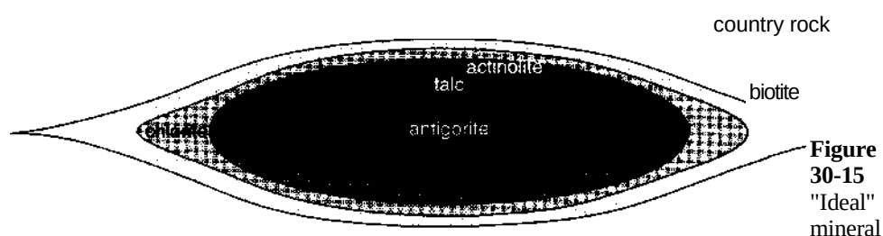
zonation due to metasomatism in < 3 -m-long ultramafic pods in low-grade regionally metamorphosed pelites at Unst, Shetland Islands. After Read (1934).
