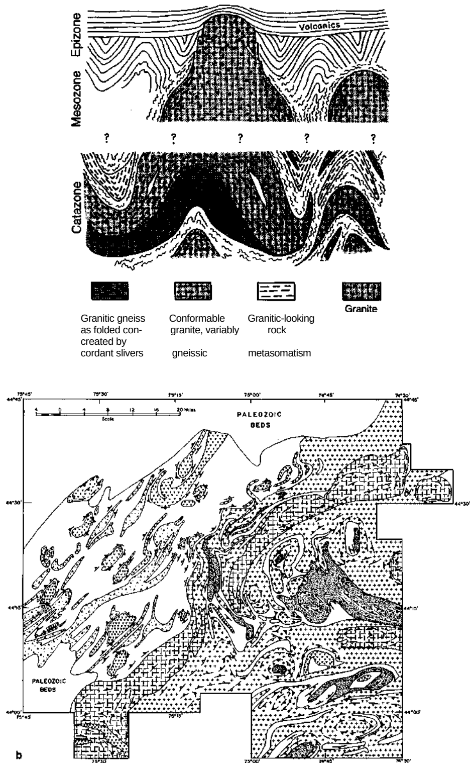
Figure 4-31 (a) General characteristics of plutons in the epizone, mesozone, and catazone. (b) Shape of concordant igneous bodies typical of the catazone, northwest Adirondacks, NY. The blank areas are metamorphic country rocks, and the patterned areas are various plutons. From Buddington (1959). Copyright © The Geological Society of America, Inc.
