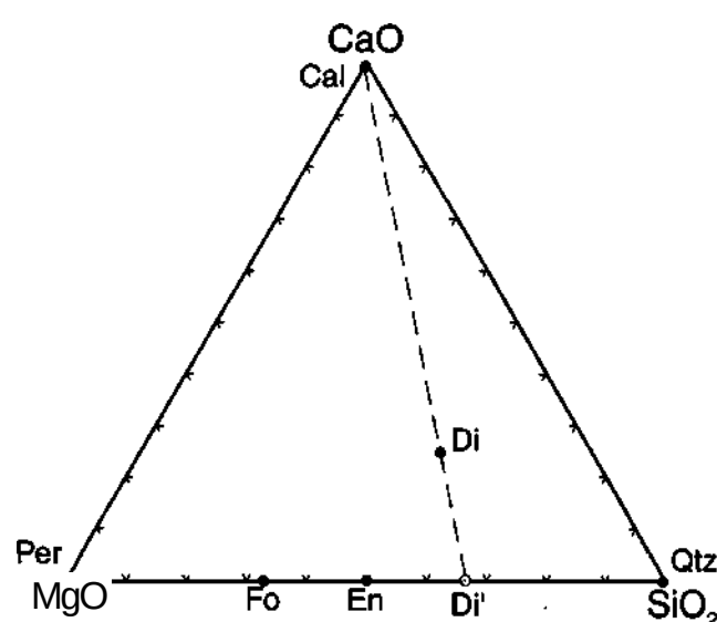
Figure 24-8 Chemographic relationships in a portion of the \text{CaO-MgO-SiO}_2 system. Di is projected from \text{CaO} to the \text{MgO-SiO}_2 base.
