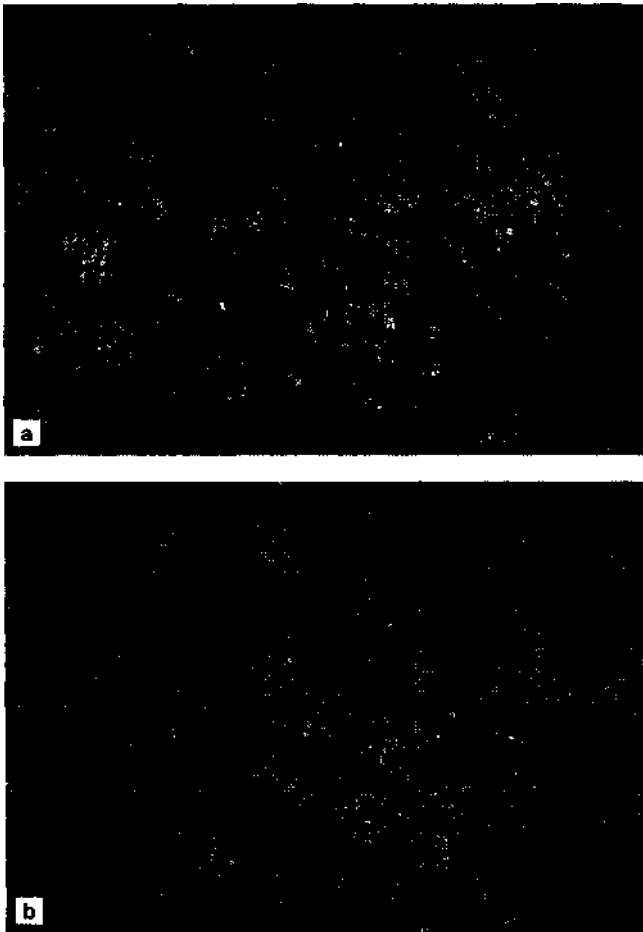
Figure 20-1 (a) "Snowflake" clusters of plagioclase crystals. (b) Typical texture of Archean anorthosite. Both from the Fiskenaesset complex, W. Greenland (a. Myers, 1985; b. Photo courtesy John Myers). Copyright Geological Survey of Denmark and Greenland.
