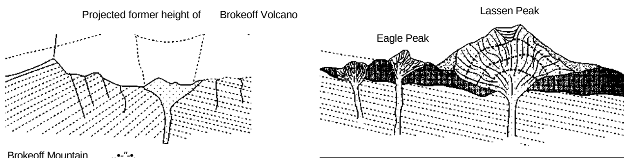
Figure 4-4 Schematic cross section of the Lassen Peak area. After Williams (1932).
