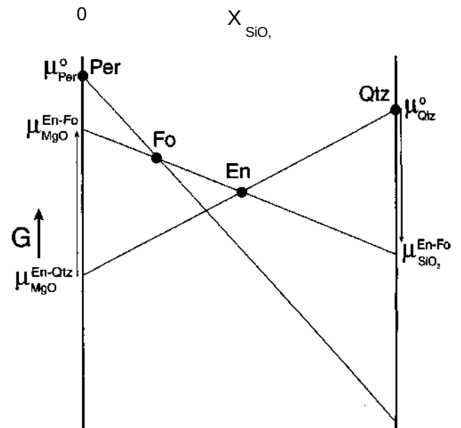
Figure 30-8 Schematic G - X_{\text{SiO}_2} diagram for the SiO 2 -MgO system at fixed temperature and pressure. See text for discussion.
