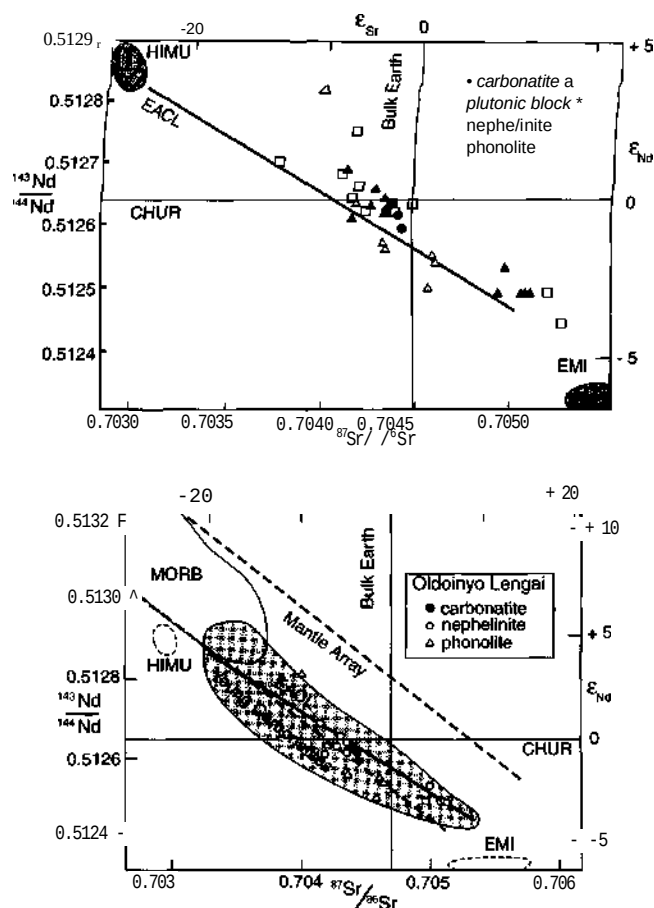
Figure 19-12 Initial ^{143}\text{Nd}/^{144}\text{Nd} vs. ^{87}\text{Sr}/^{86}\text{Sr} diagram for young carbonatites (dark shaded), and the East African Carbonatite Line (EACL), plus the HIMU and EMI mantle reservoirs (from Bell and Blenkinsop, 1987, 1989). Also included are the data for Oldoinyo Lengai natrocarbonatites and alkali silicate rocks (from Bell and Dawson, 1995). Copyright © with permission from Springer-Verlag. MORB values and the Mantle Array are from Figure 10-15.
