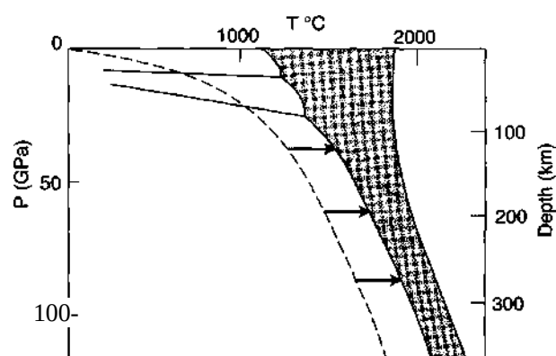
Figure 10-3 Melting by raising the temperature.
