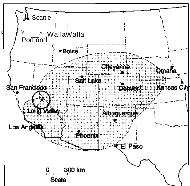
Figure 4-17 Maximum aerial extent of the Bishop ash fall deposit erupted at Long Valley 700,000 years ago. After Miller et al. (1982).
