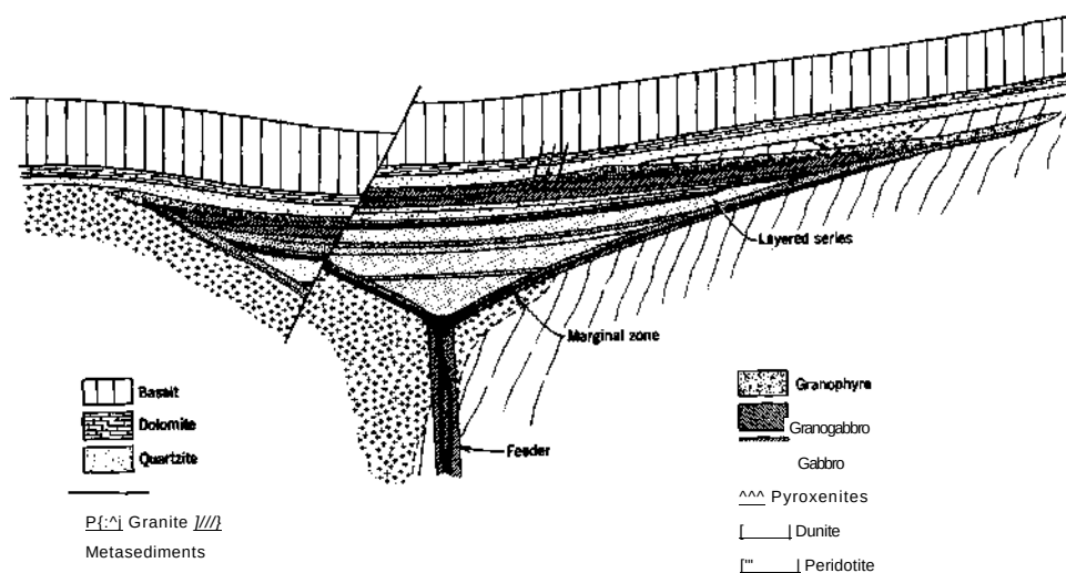
Figure 12-1 Simplified cross section of the Muskox intrusion of Canada. From Irvine and Smith (1967). Copyright © reprinted by permission of John Wiley & Sons, Inc.
