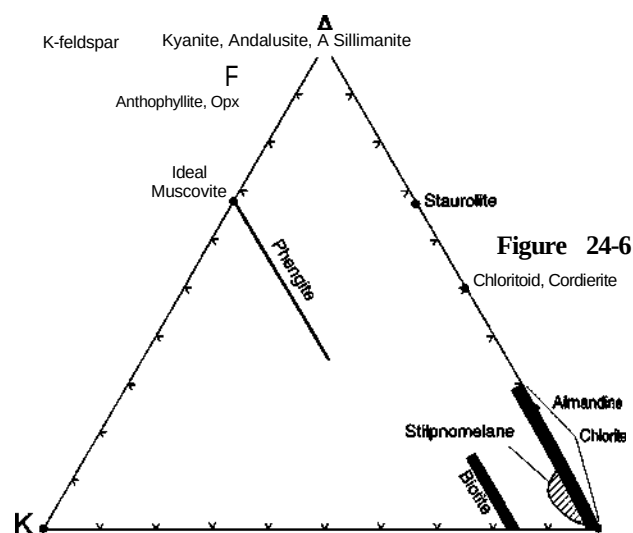
Chemographics of the AKF diagram showing the location of the ideal compositions of various common metamorphic minerals. After Ehlers and Blatt (1982).
