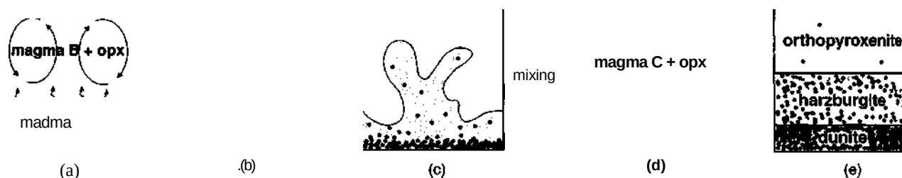
Figure 12-20 Schematic illustration of a model for the development of a cyclic unit in the Ultramafic Zone of the Stillwater Complex by influx of hot primitive magma into cooler, more evolved magma. From Raedeke and McCallum (1984). Reprinted by permission of Oxford University Press.
