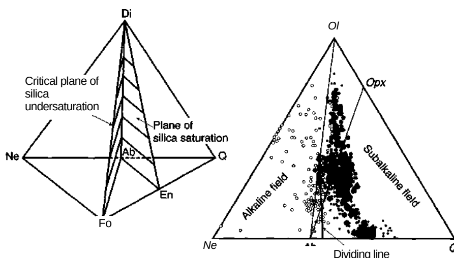
Figure 8-12 Left: the basalt tetrahedron (after Yoder and Tilley, 1962). Right: the base of the basalt tetrahedron using cation normative minerals, with the compositions of subalkaline rocks (black) and alkaline rocks (gray) from Figure 8-11, projected from Cpx. After Irvine and Baragar (1971).
