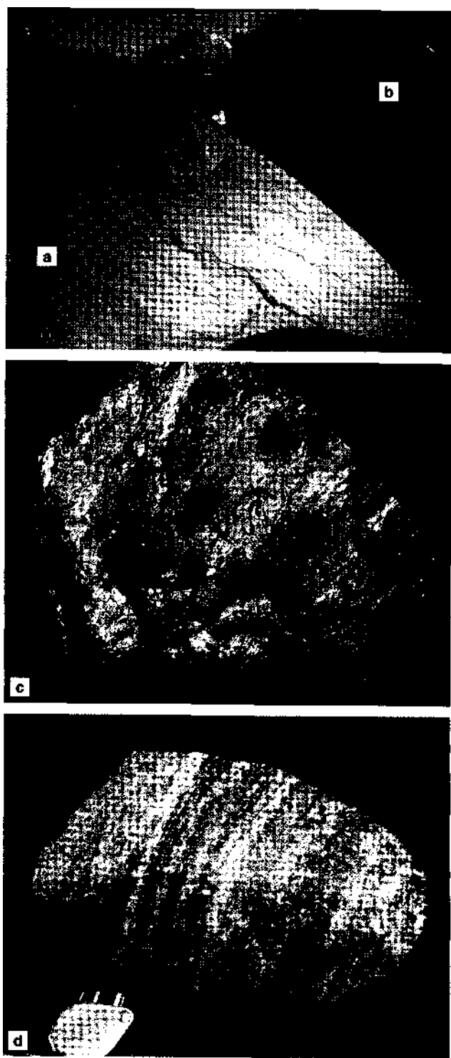
Figure 22-1 Examples of foliated metamorphic rocks, (a) Slate, (b) Phyllite. Note the difference in reflectance on the foliation surfaces between a and b: phyllite is characterized by a satiny sheen, (c) Garnet muscovite schist. Muscovite crystals are visible and silvery, garnets occur as large dark porphyroblasts. (d) Quartzofeldspathic gneiss with obvious layering.
