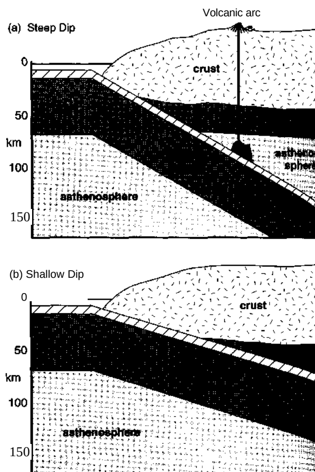
Figure 17-2 Schematic diagram to illustrate how a shallow dip of the subducting slab can pinch out the asthenosphere from the overlying mantle wedge.
