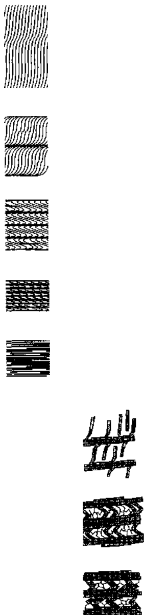
Figure 23-25 Stages in the development of crenulation cleavage as a function of temperature and intensity of the second deformation. From Passchier and Trouw (1996). Copyright © with permission from Elsevier Science.
