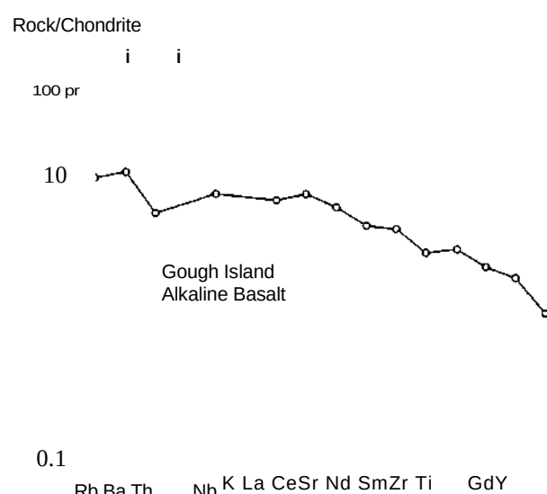
Figure 9-6 Chondrite-normalized spider diagram showing the trace element patterns of an alkaline island basalt from Gough Island (Sun and MacDonald, 1989).
