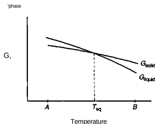
Figure 5-3 Relationship between Gibbs free energy and temperature for the solid and liquid forms of a substance at constant pressure. T_{\text{eq}} is the equilibrium temperature.
