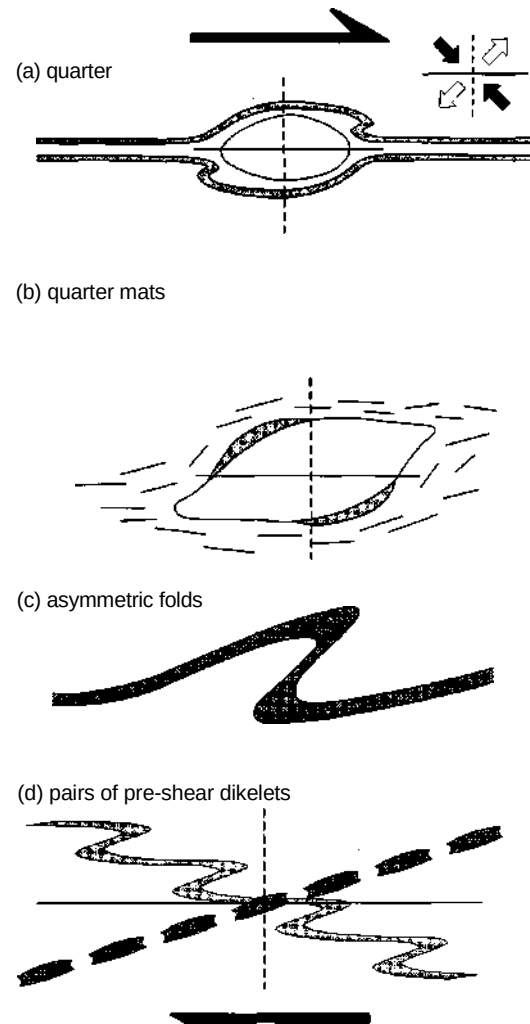
Figure 23-20 Other methods to determine sense-of-shear.
