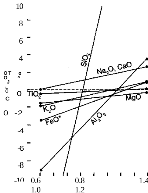
Figure 30-13 "Gresens-type" variation diagram showing the gains or losses (in grams per 100 grams of original rock A) as a function of the volume factor, f_v , in eq. (30-13). Rock A is a garnet phyllite from Stavanger, Norway, and rock B is a meta-somatized albite schist, supposedly derived from (A) After some cases this approach may indicate a Gre-sens (1967). Copyright © with permission from f Elsevier Science.
