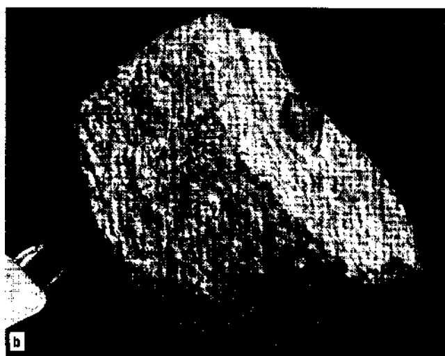
(a) Nodular texture of cordierite porphyroblasts developed during a thermal overprinting of previous regional metamorphism (note the foliation in the opaques). From Bard (1986), approx. 1.5 x 2 mm. Copyright © by permission Kluwer Academic Publishers, (b) Spotted phyllite in which small porphyroblasts of cordierite (and one larger pyrite) develop in a preexisting phyllite.
