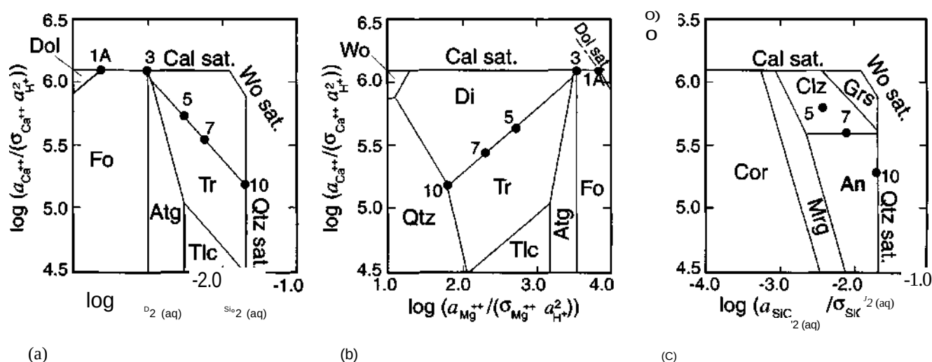
Figure 30-29 (a) \log a_{\text{CaO}} - \log a_{\text{SiO}_2} and (b) \log a_{\text{CaO}} - \log a_{\text{MgO}} diagrams in the system \text{CaO-MgO-SiO}_2\text{-H}_2\text{O-CO}_2 . (c) \log a_{\text{CaO}} - \log a_{\text{SiO}_2} diagram for the same system + \text{Al}_2\text{O}_3 , all at 425°C, 0.05 GPa, and X_{\text{CO}_2} = 0.007 . Numbered points correspond to the index numbers in Figure 30-27. After Frisch and Helgeson (1984). Reprinted by permission of the American Journal of Science.
