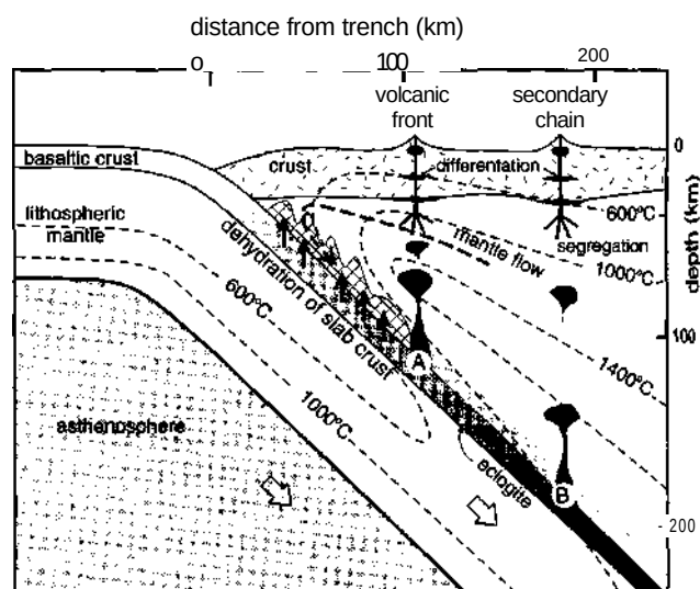
Figure 16-17 A proposed model for subduction zone magmatism with particular reference to island arcs. Dehydration of slab crust causes hydration of the mantle (hatched), which undergoes partial melting as amphibole (a) and phlogopite (b) dehydrate. From Tatsumi (1989), Tatsumi and Eggins (1995). Reprinted by permission of Blackwell Science, Inc.
