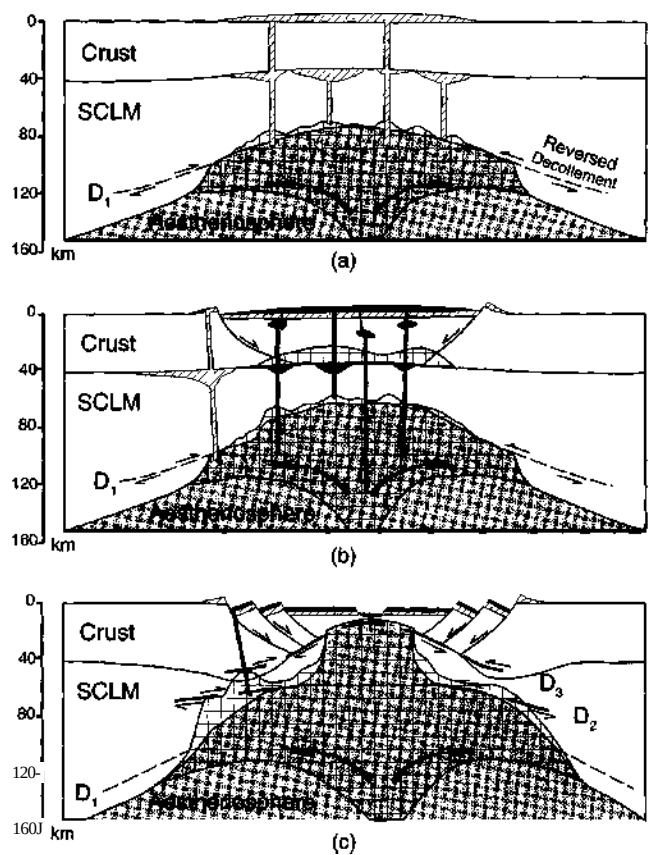
Figure 19-9 Hypothetical cross sections (same vertical and horizontal scales) showing a proposed model for the progressive development of the East African Rift System, (a) Pre-rift stage, in which an asthenospheric mantle diapir rises (forcefully or passively) into the lithosphere. Decompression melting (cross-hatches indicate areas undergoing partial melting) produces variably alkaline melts. Some partial melting of the metasomatized sub-continental lithospheric mantle (SCLM) may also occur. Reversed decollements ( D_j ) provide room for the diapir. (b) Rift stage: development of continental rifting, eruption of alkaline magmas (black) mostly from a deep asthenospheric source. Rise of hot asthenosphere induces some crustal anatexis. Rift valleys accumulate volcanics and volcanoclastic material, (c) Afar stage, in which asthenospheric ascent reaches crustal levels. This is transitional to the development of oceanic crust. Successively higher reversed decollements ( D_2 and D_3 ) accommodate space for the rising diapir. After Kampunzu and Mohr (1991) and P. Mohr (personal communication). Copyright © with permission from Springer-Verlag.
