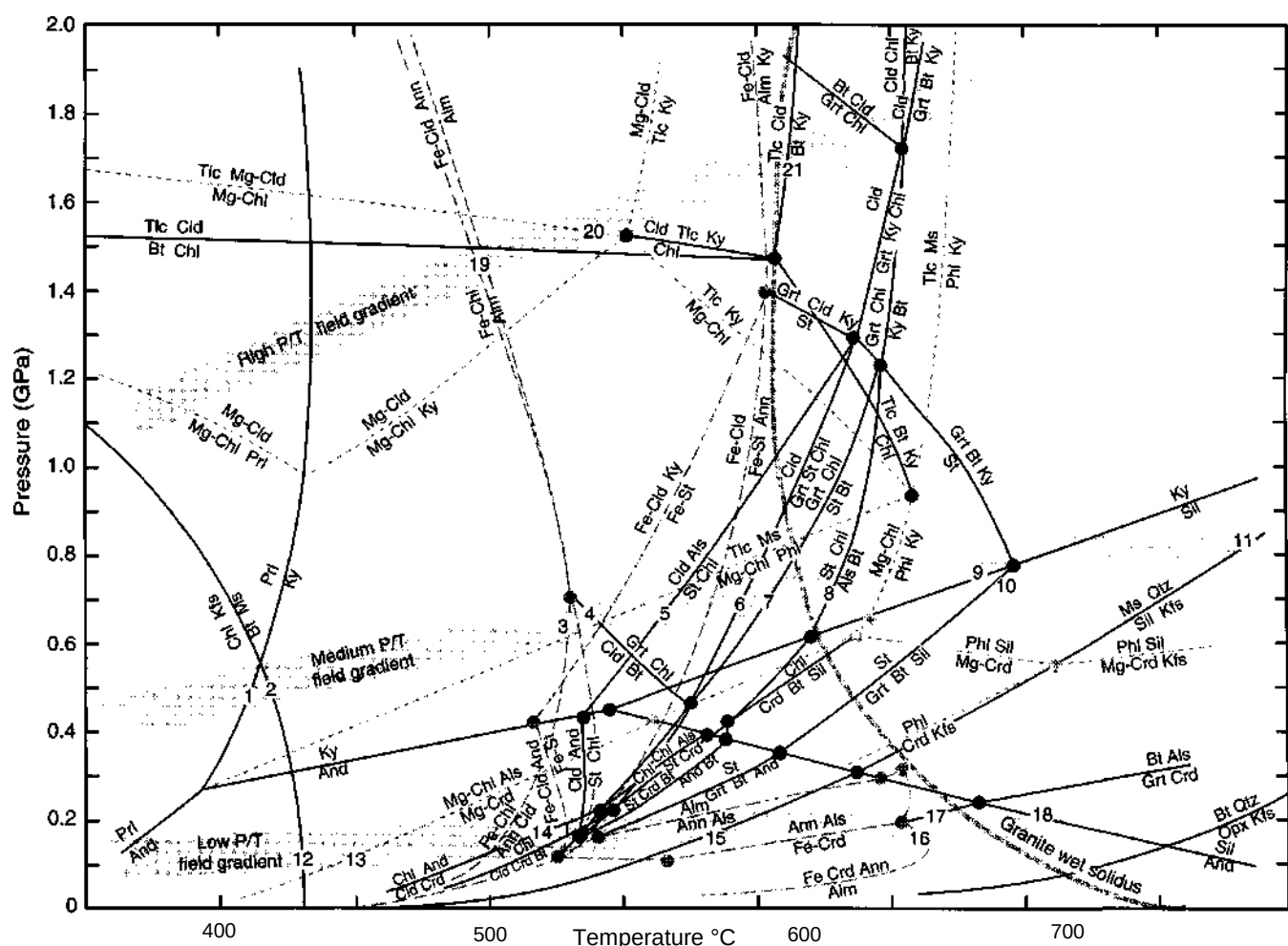
Figure 28-2 Petrogenetic grid for the system KFMASH at f_{H_2O} = -P_{tot} . Gray dashed curves represent the system KFASH and gray small-dashed curves represent the system KMASH . Reactions are not balanced, and commonly leave out quartz, muscovite, and H_2O , which are considered to be present in excess. Typical high, medium, and low P/T metamorphic field gradients are represented by broad shaded arrows. After Spear and Cheney (1989) and Spear (1999).
