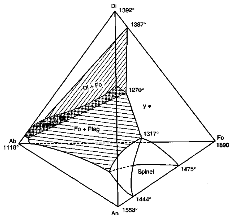
Figure 7-12 The four-component system diopside-anorthite-albite-forsterite. After Yoder and Tilley (1962). Reprinted by permission of Oxford University Press.
