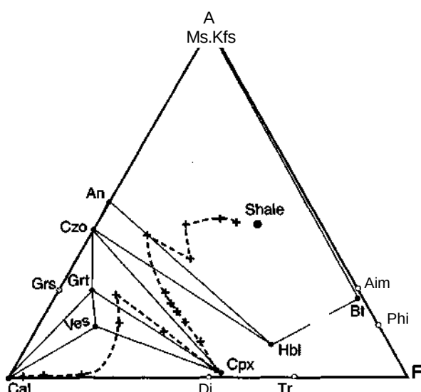
Figure 30-25 \text{Al}_2\text{O}_3 -CaO-(FeO+MgO) diagram (projected from \text{K}_2\text{O} ) showing the mineral phases and calculated bulk compositional path for metasomatic zones that develop at the contact between pelitic and carbonate layers near Lake Willoughby, VT. Ideal mineral compositions are in gray, real ones in black. After A. B. Thompson (1975). Reprinted by permission of Oxford University Press. Plus signs represent analyzed bulk-rock compositions within zones.
