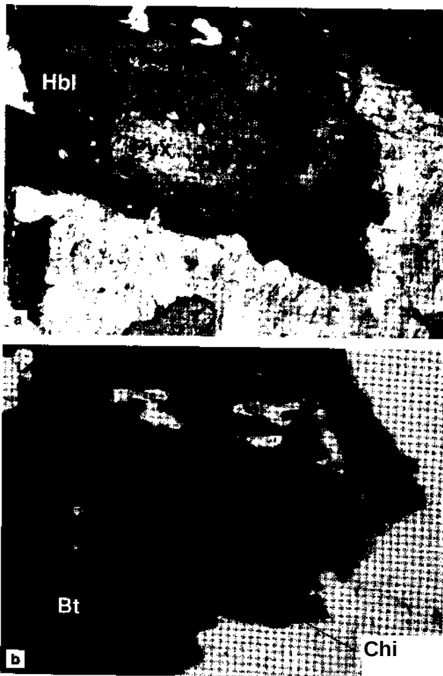
Figure 3-20 (a) Pyroxene largely replaced by hornblende. Some pyroxene remains as light areas (Pyx) in the hornblende core. Width 1 mm. (b) Chlorite (light) replaces biotite (dark) at the rim and along cleavages. Tonalite. San Diego, CA. Width 0.3 mm.
