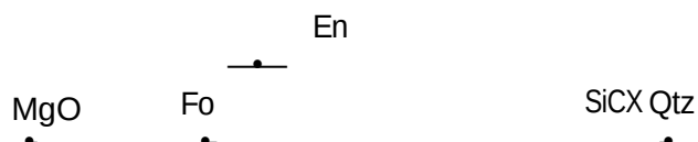
Figure 26-11 An example of a possible chemographic diagram in the binary MgO-SiO 2 system showing the positions of periclase, forsterite, enstatite, and quartz.
