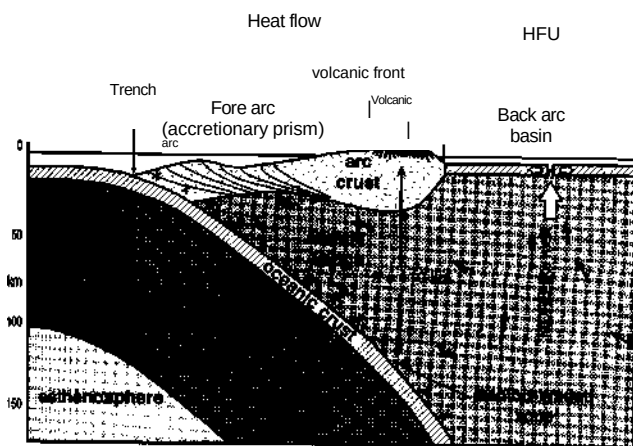
arc after Gill (1981). Copyright © with permission from Springer-Verlag. Dashed arrows in the mantle wedge represent the flow directions of McCulloch and Gamble (1991). HFU= heat flow unit ( 4.2 \cdot 10^{16} joules/cm 2 /sec). X's mark earthquake foci of the Benioff-Wadati zone.
