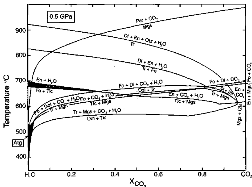
Figure 29-12 Simplified T - X_{CO_2} phase diagram for the system CaO - MgO - SiO_2 - H_2O - CO_2 at 0.5 GPa, calculated using the program TWQ of Berman (1988, 1990, 1991). The diagram focuses on ultramafic-carbonate rocks and omits reactions involving quartz. The shaded fields represent the stability ranges of, from darkest to lightest, serpentine (antigorite), anthophyllite in typical low- SiO_2 ultramafics, tremolite in low- SiO_2 ultramafics.
