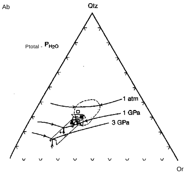
Figure 11-3 Position of the \text{H}_2\text{O} -saturated ternary eutectic (minimum melt composition) in the albite-orthoclase-silica system at various pressures. The shaded portion represents the composition of most granites. Included are the compositions of the Tuolumne Intrusive Series (Figure 4-30), with the arrow showing the direction of the trend from early to late magma batches. Experimental data from Wyllie et al. (1976).
