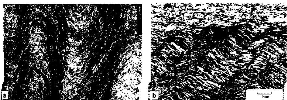
Figure 23-24 Crenulation cleavages.
