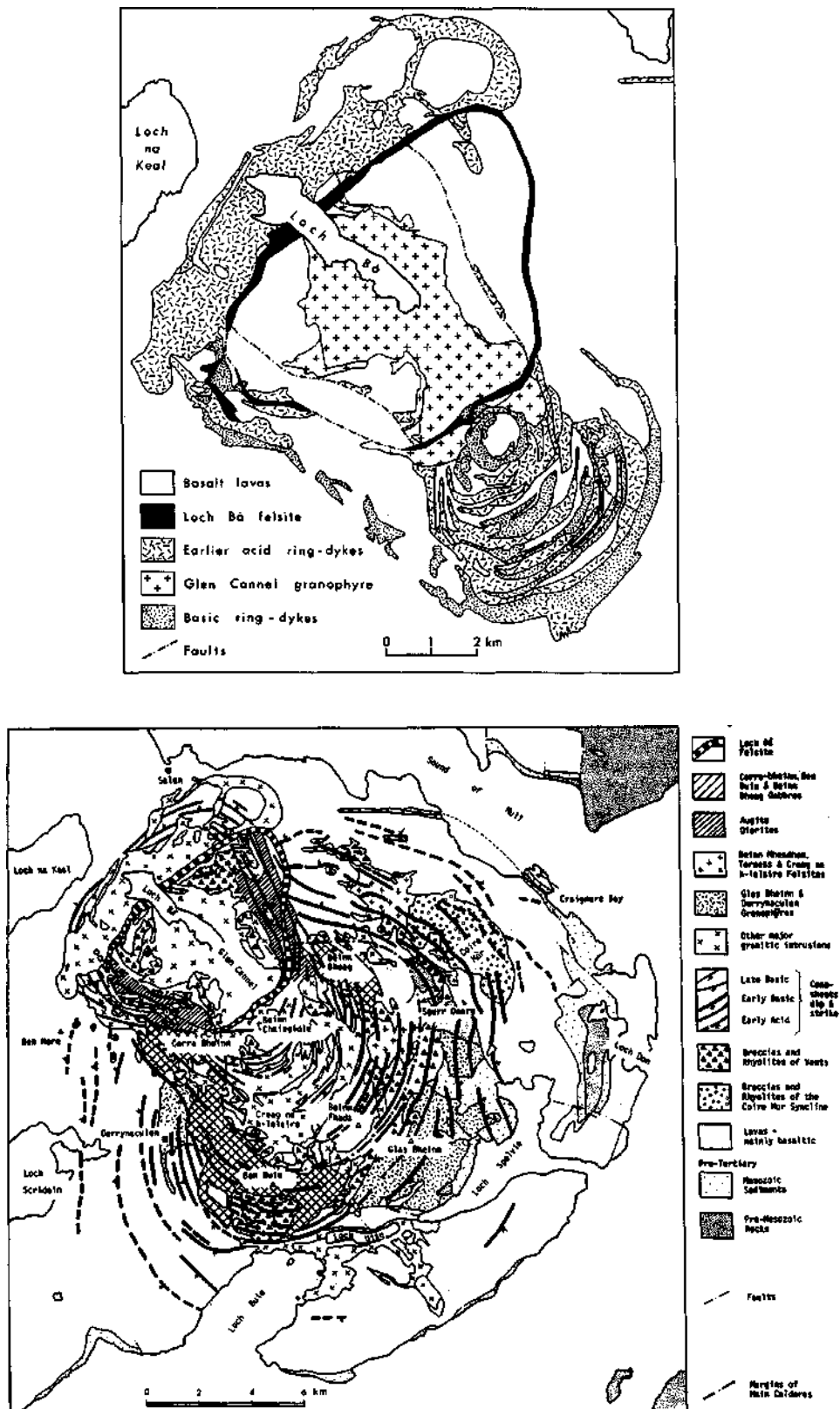
Figure 4-24 (a) Map of ring dikes, Island of Mull, Scotland. After Bailey et al. (1924). (b) Cone sheets in the same area of Mull, after Ritchey (1961). Note that the black felsite ring dike in part (a) is shown as the striped ring in the NW of part (b). Copyright © by permission British Geological Survey.
