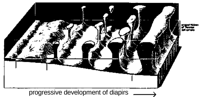
Figure 4-33 Block diagram of subsurface salt diapirs in Northern Germany. After Trusheim (1960). AAPG ©, reprinted by permission of the AAPG.
