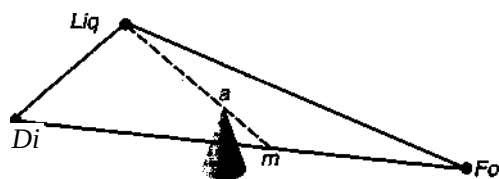
Figure 7-3 Diagram to illustrate the derivation of the relative amounts of three phases coexisting with a given bulk composition ( a ).
