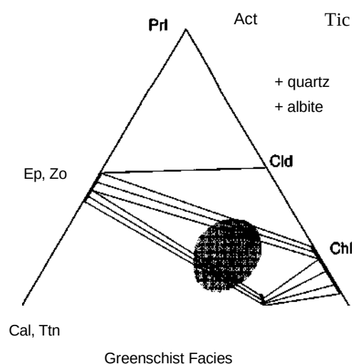
Figure 25-6 A CF diagram illustrating representative mineral assemblages for metabasites in the greenschist facies. The composition range of common mafic rocks is shaded.
