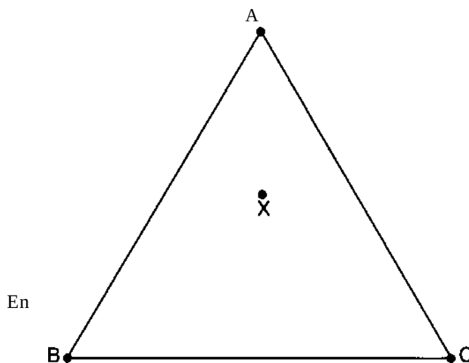
Figure 26-12 A hypothetical three-component system A - B - C having a compound X within the triangle. X can be generated by a reaction involving A + B + C .
