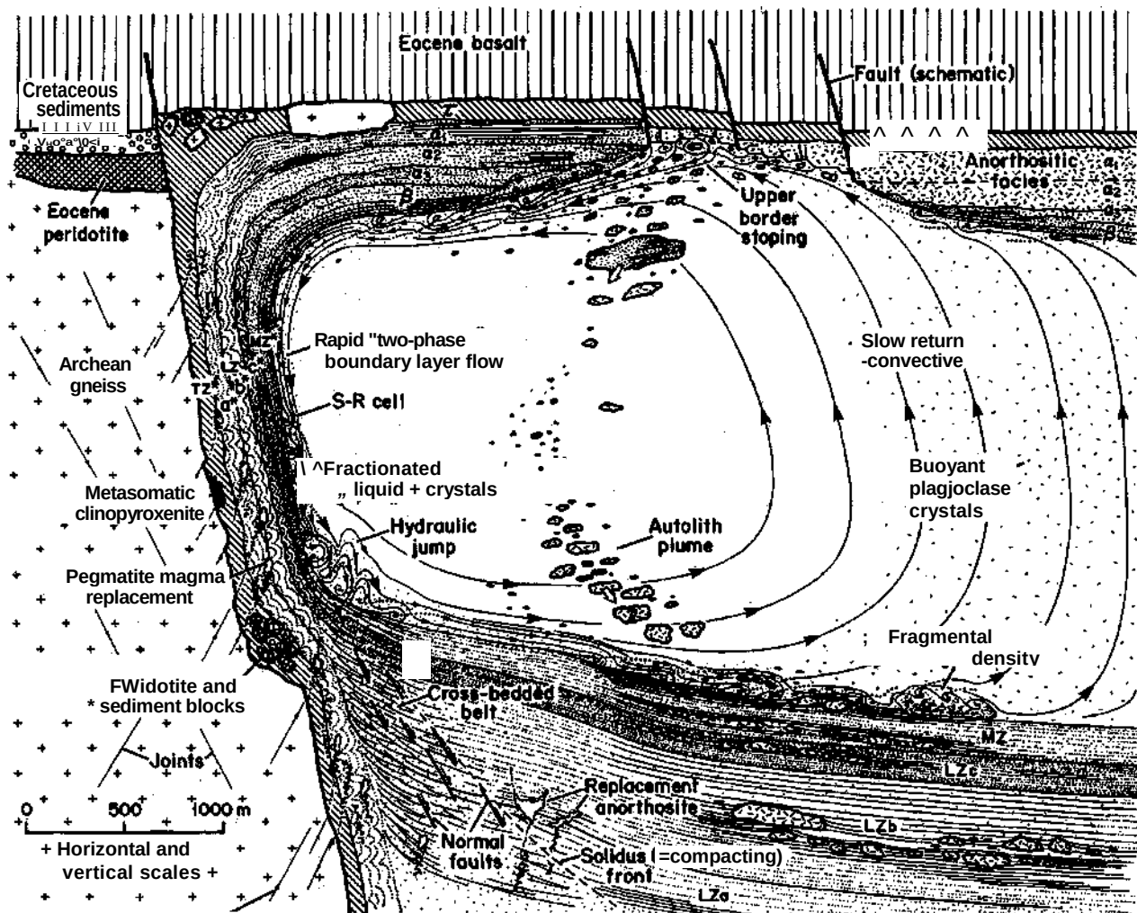
Figure 12-17 Schematic synthesis of the processes believed to be occurring in the Skaergard magma chamber early in the Middle Zone stage of development. Density driven "S-R" vortex cells descend along the sloping roof and walls to spread across the floor, producing rhythmic layers which may be graded on the floor. Occasional larger density surge deposits result from slumps originating along the walls. Blocks of autoliths and xenoliths are also broken from the walls and roof, and impact the floor. Compaction of cumulates below the floor release liquids that react with the overlying layers to form cross-cutting replacement anorthosite. From Irvine et al. (1998). Copyright © The Geological Society of America, Inc.
