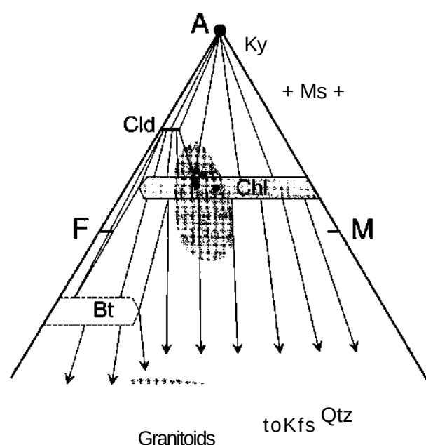
Figure 28-5 A FM projection for the biotite zone, greenschist facies , above the chloritoid isograd. The compositional ranges of common pelites and granitoids are shaded.
