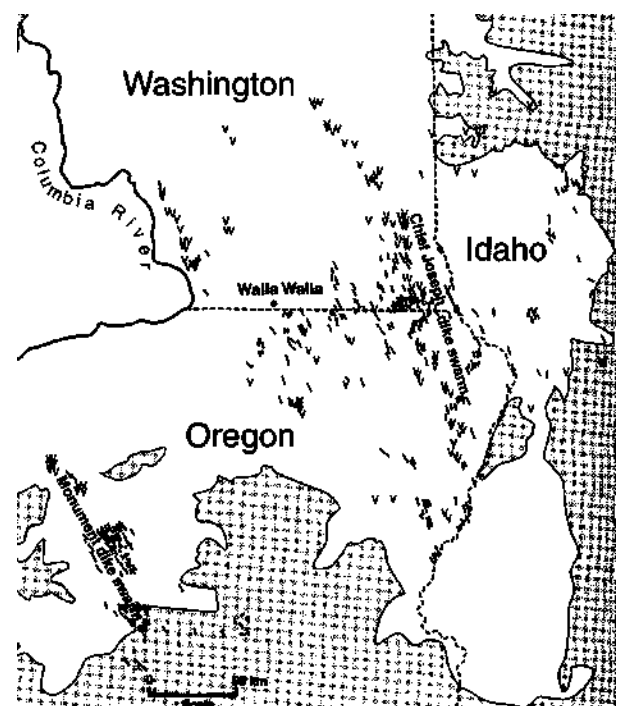
Figure 4-10 Location of the exposed feeder dikes (heavy lines) and vents (V's) of the southeastern portion of the Columbia River Basalts. Unshaded area covered by CRB. After Tolan et al. (1989). Copyright © The Geological Society of America, Inc.
