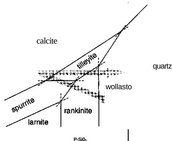
Figure 30-24 Schematic isothermal isobaric \mu_{\text{CO}_2} - \mu_{\text{H}_2\text{O}} diagram for fluids in the \text{CaO-SiO}_2\text{-H}_2\text{O} system at high temperatures. After Joesten (1974). Reprinted by permission of the American Journal of Science.
