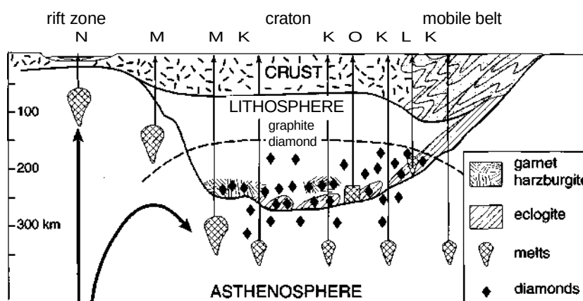
Figure 19-21 Hypothetical cross section of an Archean craton with an extinct ancient mobile belt (once associated with subduction) and a young rift. The low cratonic geotherm causes the graphite-diamond transition to rise in the central portion. Lithospheric diamonds therefore occur only in the peridotites and eclogites of the deep cratonic root, where they are then incorporated by rising magmas (mostly kimberlitic-"K"). Lithospheric orangeites ("O") and some lamproites ("L") may also scavenge diamonds. Melilitites ("M") are generated by more extensive partial melting of the asthenosphere. Depending on the depth of segregation they may contain diamonds. Nephelinites ("N") and associated carbonatites develop from extensive partial melting at shallow depths in rift areas. After Mitchell (1995). Copyright © by permission Kluwer Academic Publishers.
