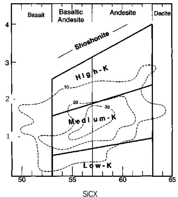
Figure 16-4 The three andesite series of Gill (1981). A fourth very high K shoshonite series is rare. Contours represent the concentration of 2500 analyses of andesites stored in the large
