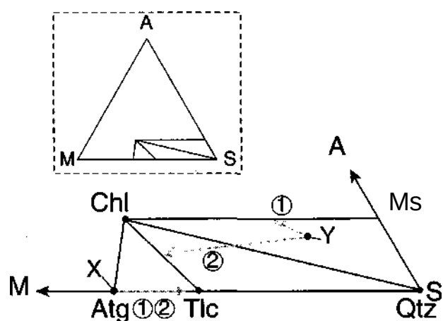
Figure 30-17 AMS diagram ( A = \text{Al}_2\text{O}_3 , M = \text{MgO} + \text{FeO} , and S = \text{SiO}_2 ), projected from \text{K}_2\text{O} , for ideal lower-temperature metasomatic zones around ultramafic bodies. After Brady (1977).
