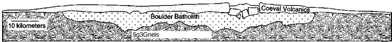
Figure 4-36 Diagrammatic cross section of the Boulder Batholith, Montana, prior to exposure. After Hamilton and Myers (1967).
