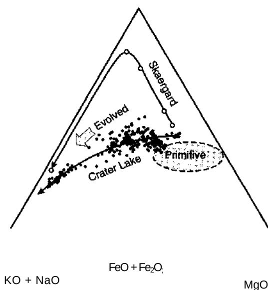
Figure 8-3 AFM diagram for Crater Lake volcanics (data from Figure 8-2) and the Skaergard
