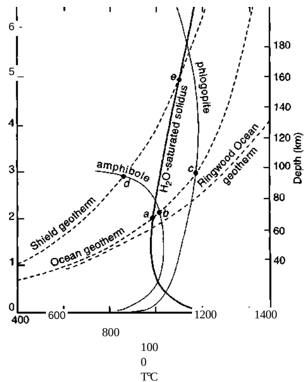
Figure 10-6 Phase diagram (partly schematic) for a hydrous mantle system, including the \text{H}_2\text{O} -saturated Iherzolite solidus of Kushiro et al. (1968), the dehydration breakdown curves for amphibole (Millhollen et al., 1974) and phlogopite (Modreski and Boettcher, 1973), plus the ocean and shield geotherms of Clark and Ringwood (1964) and Ringwood (1966). After Wyl-lie (1979). Copyright © reprinted by permission of Princeton University Press.
