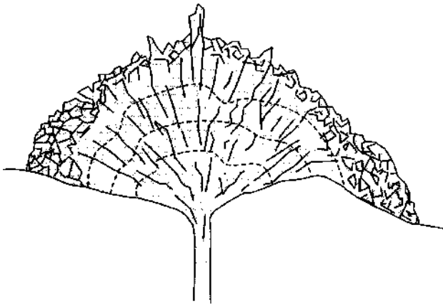
Figure 4-7 Schematic cross section through a lava dome.
