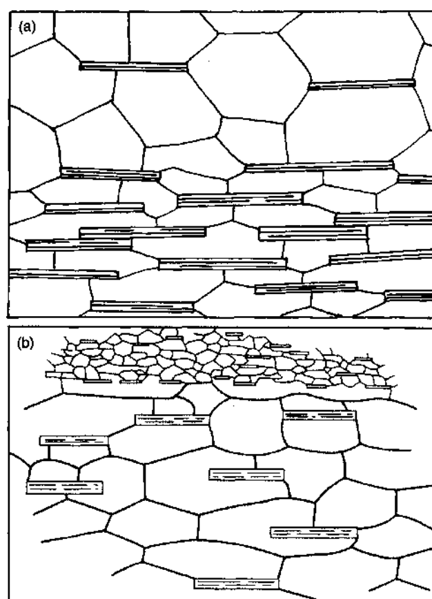
Figure 23-11 Drawings of quartz-mica schists, (a) Closer spacing of micas in the lower half causes quartz grains to passively elongate in order for quartz-quartz boundaries to meet mica (001) faces at 90^\circ . From Shelley (1993). (b) Layered rock in which the growth of quartz has been retarded by grain boundary "pinning" by finer micas in the upper layer. From Vernon (1976).
