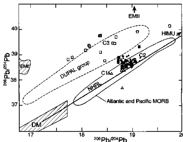
Figure 15-12 ^{208}\text{Pb}/^{204}\text{Pb} vs. ^{206}\text{Pb}/^{204}\text{Pb} for the basalts of the CRBG. Included for reference are EMI, EMU, the DUPAL group, the MORE array, and the NHRL (northern hemisphere reference line) connecting DM and HIMU mantle reservoirs from Figure 14-6. Symbols as in Figure 15-11.
