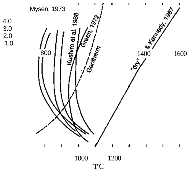
Figure 10-5 Dry peridotite solidus compared to several experiments on \text{H}_2\text{O} -saturated peridotites.
