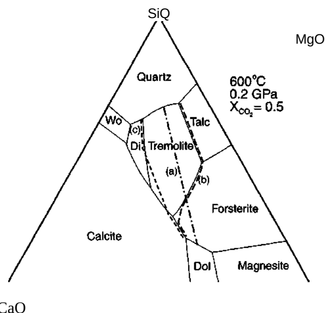
Figure 30-26 Schematic CaO-MgO-SiO 2 -CO 2 -H 2 O diagram showing the composition of the fluid solution in equilibrium with the phases shown at approximately 600°C and 0.2 GPa (projected from H 2 O and CO 2 at a constant 1:1 ratio). After Frantz and Mao (1976). Reprinted by permission of the American Journal of Science.
