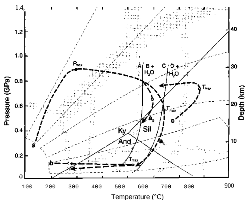
figure 25-12 Schematic pressure-temperature-time paths based on heat-flow models for (a) crustal thickening, (b) shallow magmatism, and (c) some types of granulite facies metamorphism. Al 2 SiO 5 phase diagram and two hypothetical dehydration curves are included. Open circles represent maximum temperatures attained. Facies boundaries, and facies series from Figures 25-2 and 25-3.
