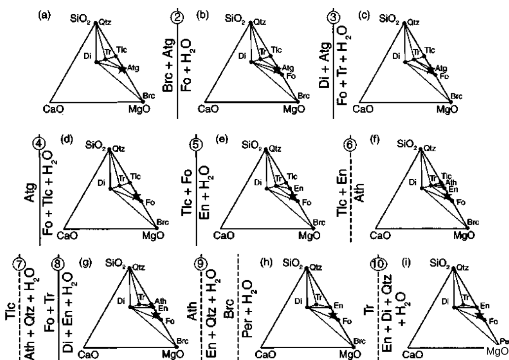
Figure 29-11 Chemographics of ultramafic rocks in the CMS-H system (projected from \text{H}_2\text{O} ) showing the stable mineral assemblages (in the presence of excess \text{H}_2\text{O} ) and changes in topology caused by reactions along the medium P/T metamorphic field gradient illustrated in Figure 29-10. The star represents the composition of a typical mantle Iherzolite. Dashed reactions represent those that do not occur in typical ultramafic rocks, but rather in unusually \text{SiO}_2 -rich or \text{SiO}_2 -poor varieties. After Spear (1993).
