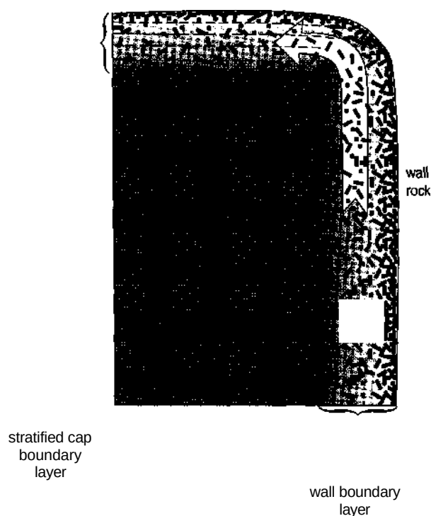
Figure 11-12 Formation of boundary layers along the walls and top of a magma chamber. Gradients in temperature result in variations in extent of crystallization, which, in turn, creates a compositional gradient in the interstitial liquid. The liquid composition varies from that of the original magma in the interior to highly evolved at the margin where crystallization is advanced. The evolved liquid is less dense, and may rise to spread out at the top, forming a stagnant cap layer.
