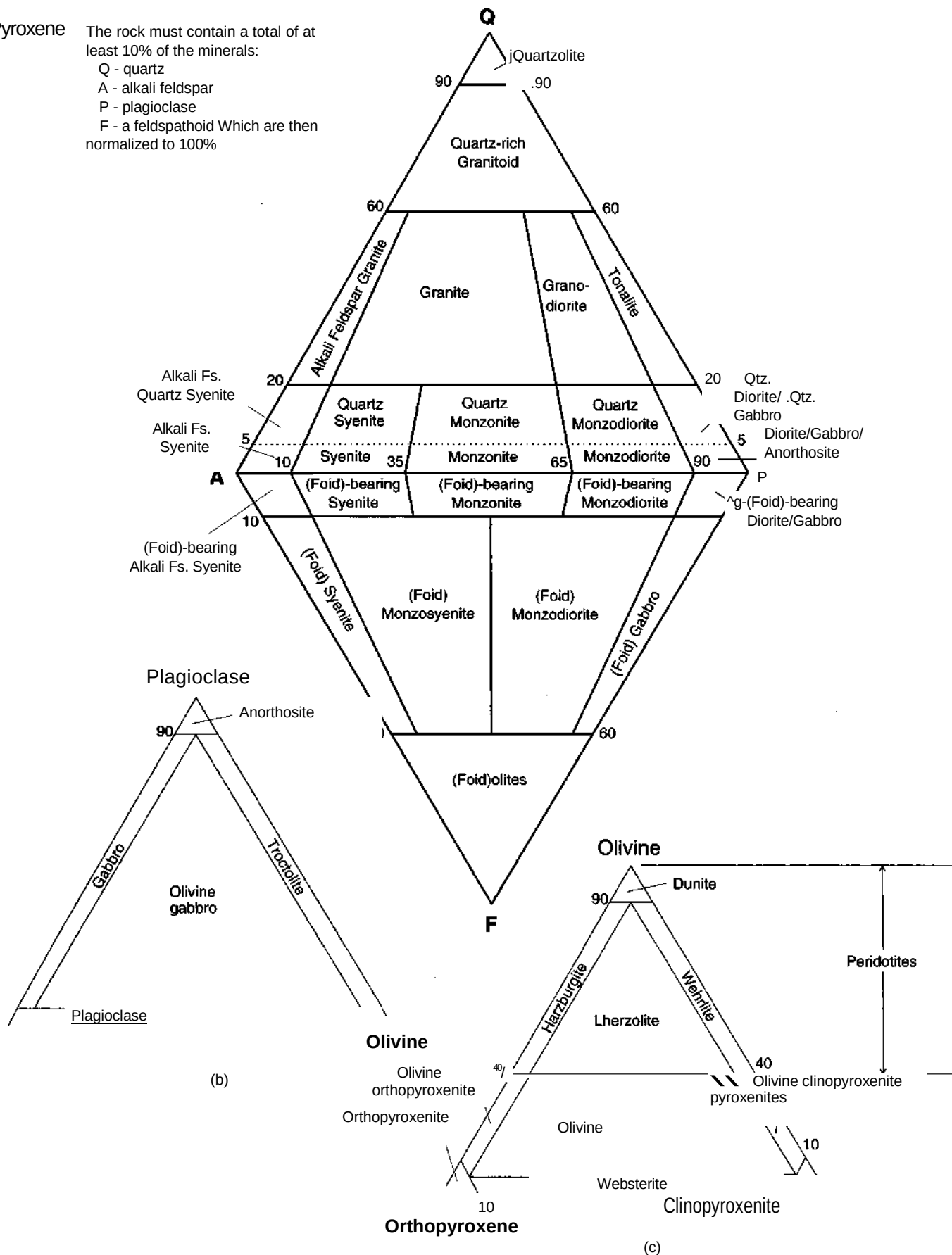
Figure 2-2 A classification of the phaneritic igneous rocks, (a) Phaneritic rocks with more than 10% (quartz + feldspar + feldspathoids). (b) Gabbroic rocks, (c) Ultramafic rocks. After IUGS (see references at the end of the chapter).
