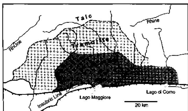
Figure 29-5 Metamorphic zones developed in regionally metamorphosed dolomitic rocks of the Lepontine Alps, along the Swiss-Italian border. After Trommsdorff (1966, 1972).
