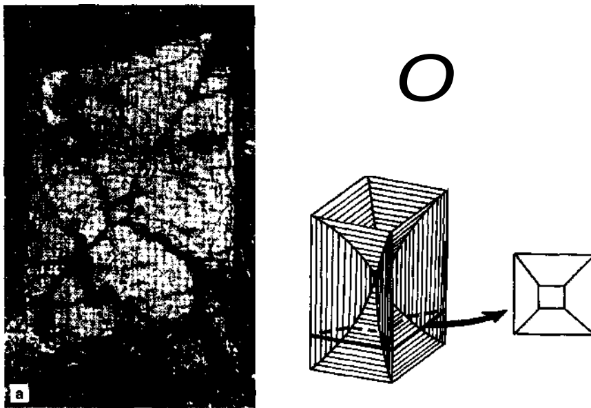
Figure 23-50 Chiastolite cross in andalusite and Frondel's (1934) theory for its development. From Shelley (1993). Copyright © by permission Kluwer Academic Publishers.
