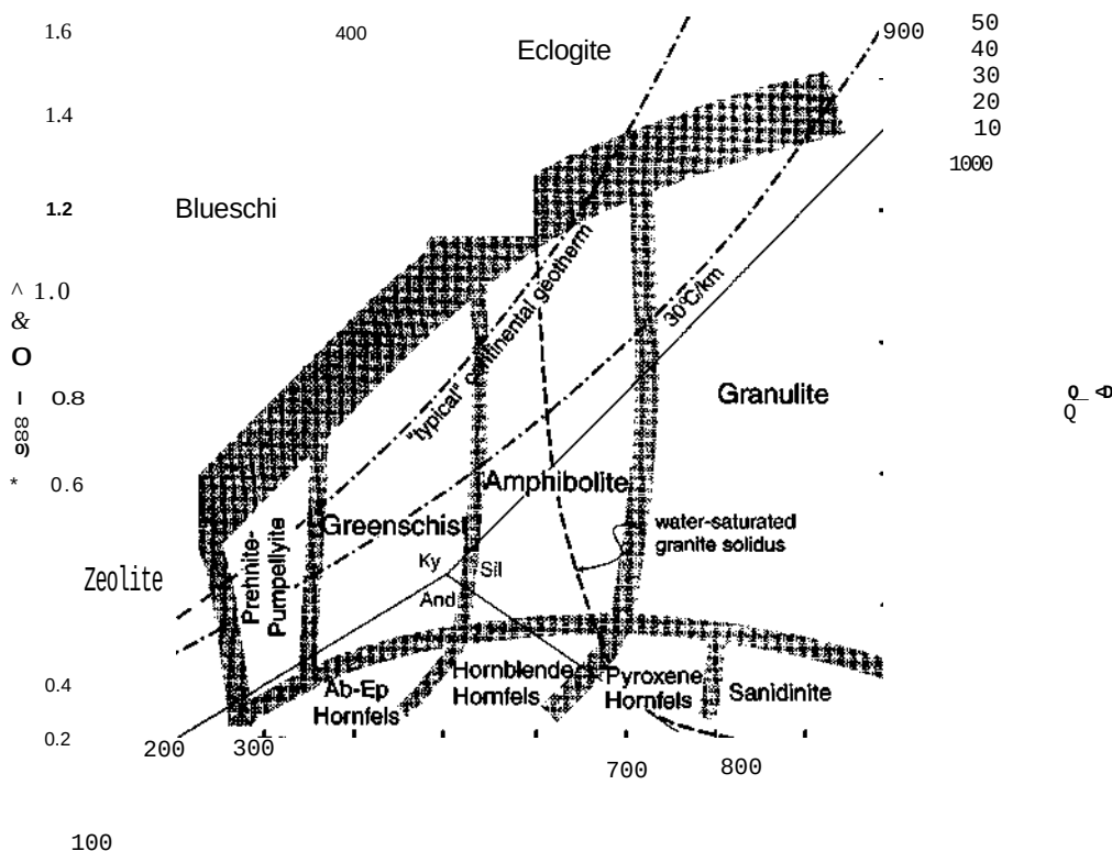
Figure 25-2 Temperature-pressure diagram showing the generally accepted limits of the various facies used in this text. Boundaries are approximate and gradational. The "typical" or average continental geotherm is from Brown and Mus (1993). The 30^{\circ}\text{C}/\text{km} geothermal gradient is an example of an elevated orogenic geothermal gradient. The stability ranges of three \text{Al}_2\text{SiO}_5 polymorphs are from Figure 21-9, and the minimum melting curve for \text{H}_2\text{O} -saturated granite is from Figure 18-10.
