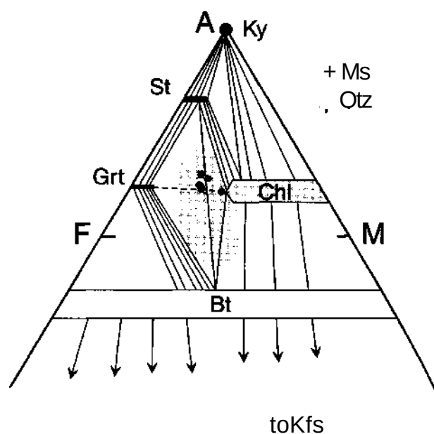
Figure 28-11 AFM diagram for the staurolite zone, amphibolite fades, showing the tie-line flip associated with reaction (28-12) which introduces staurolite into many low-Al common pelites (shaded). After Carmichael (1970). Reprinted by permission of Oxford University Press.
