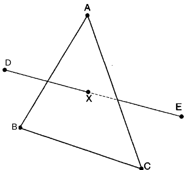
Figure 26-13 Three-dimensional perspective view of the A-B-C triangle in Figure 26-14, contained in a hypothetical four-component system. X can be generated by a combination of A + B + C or of D + E , implying a possible reaction: A + B
