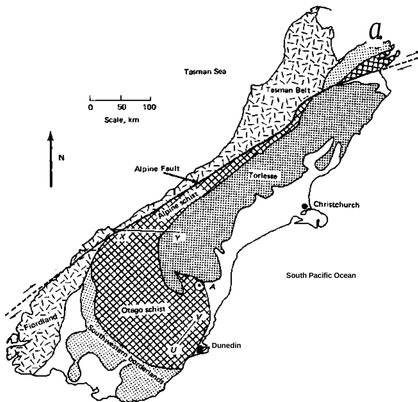
Figure 21-10 Geologic sketch map of the South Island of New Zealand showing the Mesozoic metamorphic rocks east of the older Tasman Belt and the Alpine Fault. The Torlesse Group is metamorphosed predominantly in the prehnite-pumpellyite zone, and the Otago Schist in higher grade zones. X-Y is the Haast River Section of Figure 21-11. From Turner (1981).
