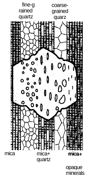
Figure 23-33 Illustration of an \text{Al}_2\text{SiO}_5 poikiloblast that consumes more muscovite than quartz, thus inheriting quartz (and opaque) inclusions. The nature of the quartz inclusions can be related directly to individual bedding substructures. Note that some quartz is consumed by the reaction, and that quartz grains are invariably rounded. From Passchier and Trouw (1996). Copyright © with permission from Elsevier Science.
