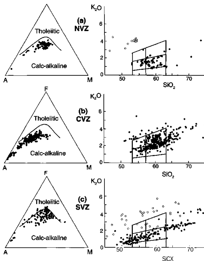
Figure 17-3 AFM and K_2O vs. SiO_2 diagrams (including Hi-K, Med.-K, and Low-K types of Gill, 1981; see Figures 16-4 and 16-6) for volcanics from the (a) northern, (b) central and (c) southern volcanic zones of the Andes. Open circles in the NVZ and SVZ are alkaline rocks. Data from Thorpe et al. (1982,1984), Geist (personal communication), Deruelle (1982), Davidson (personal communication), Hickey et al. (1986), Lopez-Escobar et al. (1981), Hormann and Pichler (1982).
