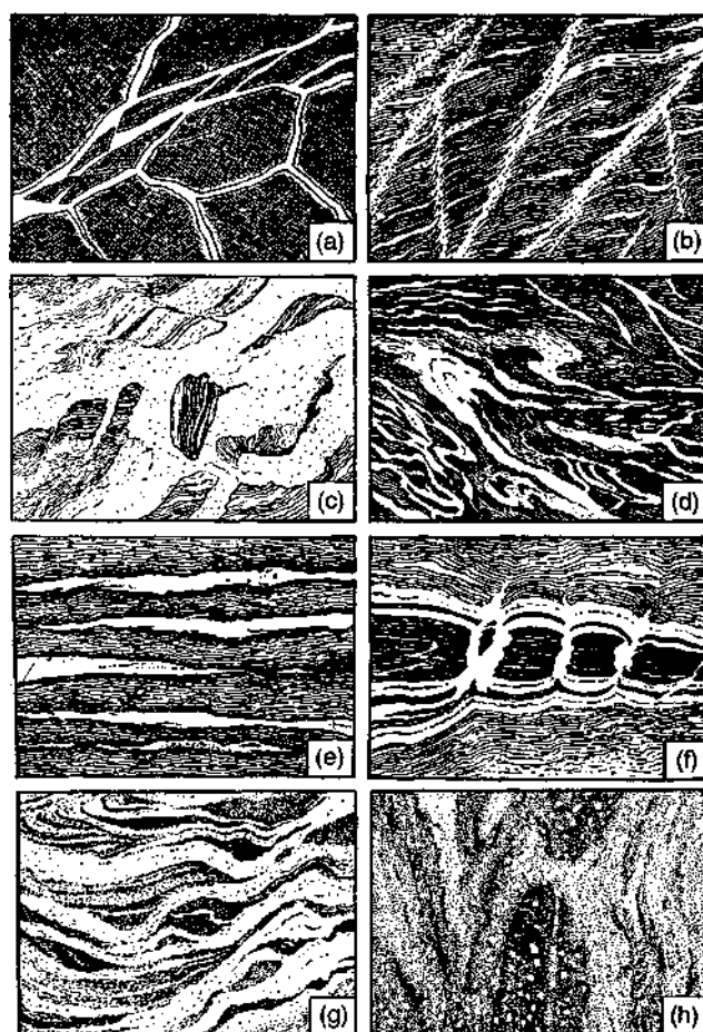
Figure 28-22 Some textures of migmatites . (a) Breccia structure in agmatite. (b) Net-like structure, (c) Raft-like structure. (d) Vein structure, (e) Stromatic, or layered, structure, (f) Dilation structure in a boudinaged layer, (g) Schleiren structure. (h) Nebulitic structure. From Mehnert (1968). Copyright © with permission from Elsevier Science.
