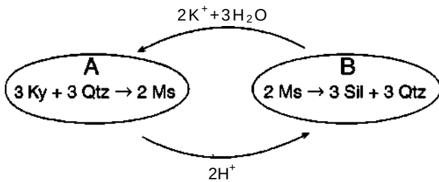
Figure 26-21 A possible mechanism by which the \text{Ky} \rightarrow \text{Sil} reaction can be accomplished while producing the textures illustrated in Figure 26-20a and b. The exchange of ions shown between the two local zones is required if the reactions are to occur. After Carmichael (1969). Copyright © with permission from Springer-Verlag.
