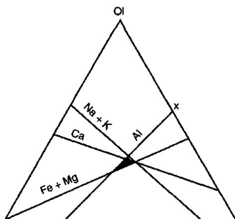
Figure 8-9 Equilateral triangle showing the solution to the bulk mineral extract (shaded area) best fitting the criteria for the variation diagrams in Figure 8-8. From Ragland (1989). Reprinted by permission of Oxford University Press.
