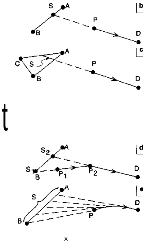
Figure 8-6 Stacked variation diagrams of hypothetical components X and Y (either weight or mol %). P = parent, D = daughter, S = solid extract, A , B , C = possible extracted solid phases. For explanation, see text. From Ragland (1989). Reprinted by permission of Oxford University Press.
