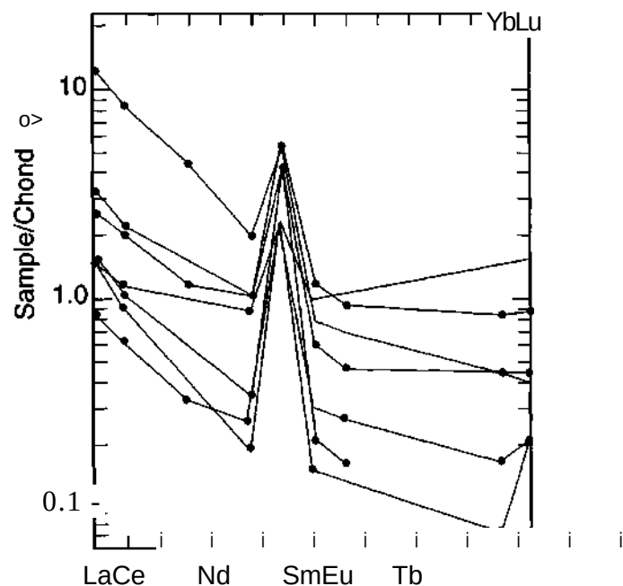
Figure 20-2 Chondrite-normalized rare earth element diagram for some typical Archean anorthosites from the Bad Vermillion (Ontario) and Fiskenaesset (Greenland) bodies. Data from Siefert et al. (1997), Simmons and Hanson (1978), and Ashwal et al. (1989).
