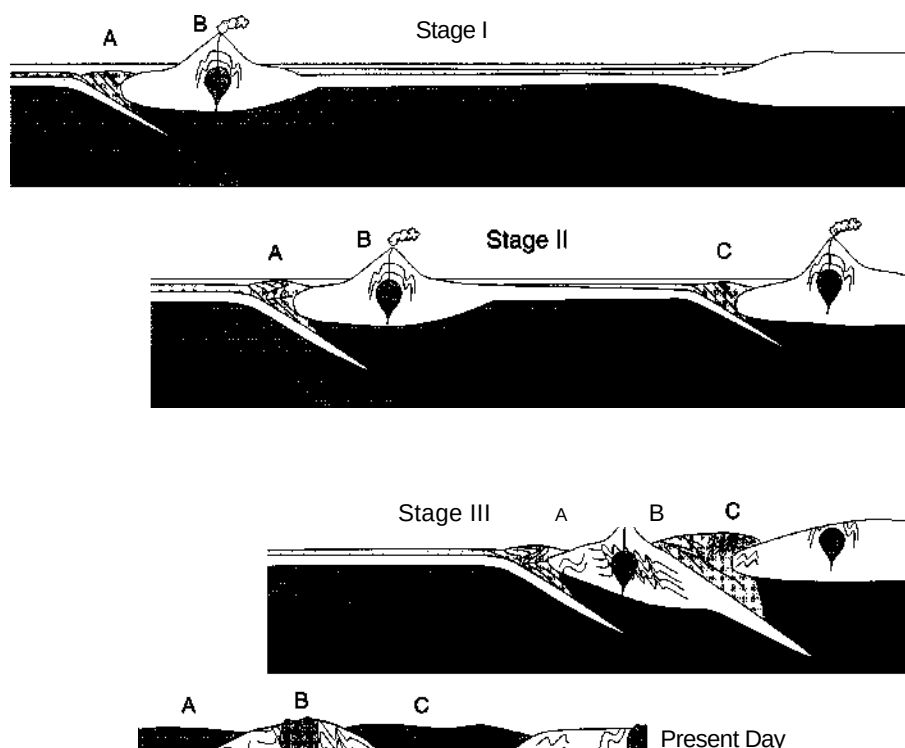
Figure 23-49 Hypothetical development of an orogenic belt involving development and eventual accretion of a volcanic island arc terrane. See the text for discussion. After Passchier and Trouw (1996). Copyright © with permission from Elsevier Science.
