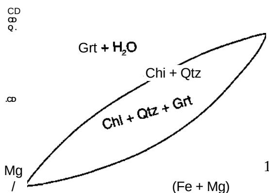
Figure 26-9 Schematic isobaric T - X_{\text{Mg}} diagram representing the simplified metamorphic reaction \text{Chi} + \text{Qtz} \rightarrow \text{Grt} + \text{H}_2\text{O} .
