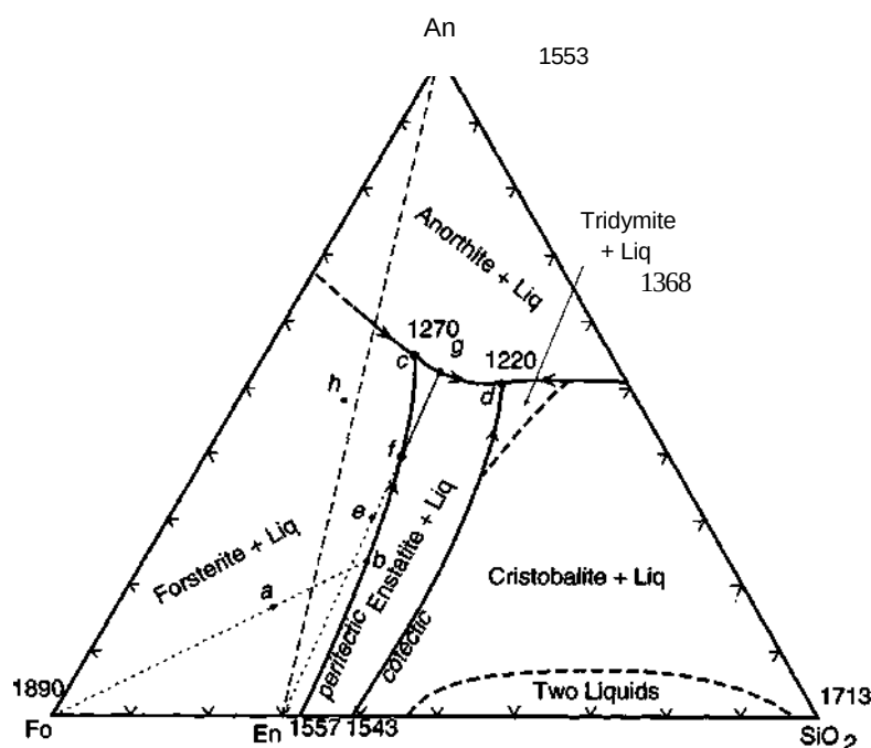
Figure 7-4 Isobaric diagram illustrating the cotectic and peritectic curves in the system forsterite-anorthite-silica at 0.1 MPa. After Anderson (1915) reprinted by permission of the American Journal of Science, and Irvine (1975).
