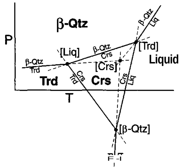
Figure 26-17 A portion of the P - T phase diagram for \text{SiO}_2 (Figure 6-6) showing two stable invariant points [Trd] and [Liq] and two metastable ones. [(3-Qtz)] occurs at negative pressure, and [Crs] is truly metastable in that it is the intersection of metastable extensions. From Spear (1993).
