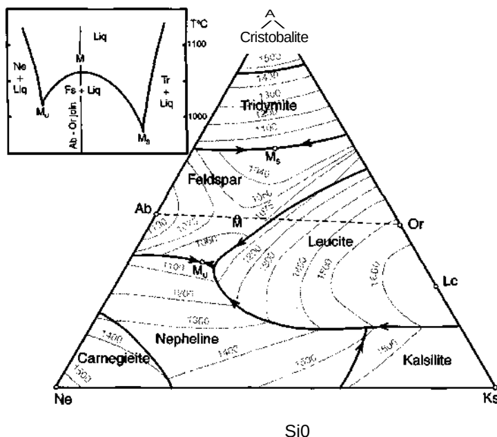
Figure 19-7 Phase diagram for the system SiO 2 -NaAl-SiO 4 -KAlSiO 4 -H 2 O at 1 atm. pressure. Insert shows a T-X section from the silica-undersaturated thermal minimum ( M_u ) to the silica-oversaturated thermal minimum ( M_s ) that crosses the lowest point ( M ) on the binary Ab-Or thermal barrier that separates the undersaturated and oversaturated zones. After Schairer and Bowen (1935) and Schairer (1950). Copyright © by the University of Chicago.
